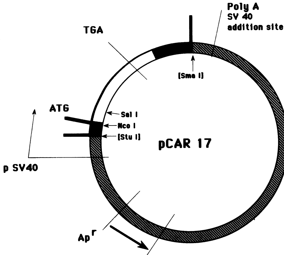
Figure 1. The vector derived from pYZ28 containing the cDNA for KB cell FBP used for the stable transfection of 3T3 cells. Hatched box : Sequence derived from pYZ28 between Stu I and Sma I sites. Open box : FBP cDNA. Solid boxes : Junction regions acquired in cloning. Abbreviations: Ap r ; ampicillin resistance gene; pSV40; SV 40 promoter. [ ]: these sites were destroyed in cloning the cDNA into this vector. The inset shows the origin of the nucleotide sequences that comprise the final vector: pYZ28 is the parent plasmid and contains the SV40 promoter and the bacteriophage T7 sequences (17, 18); the synthetic sequence contains the Nco I restriction site and the Kozak consensus sequence; pUC 18 is the derived plasmid into which the truncated FBP cDNA was cloned.
