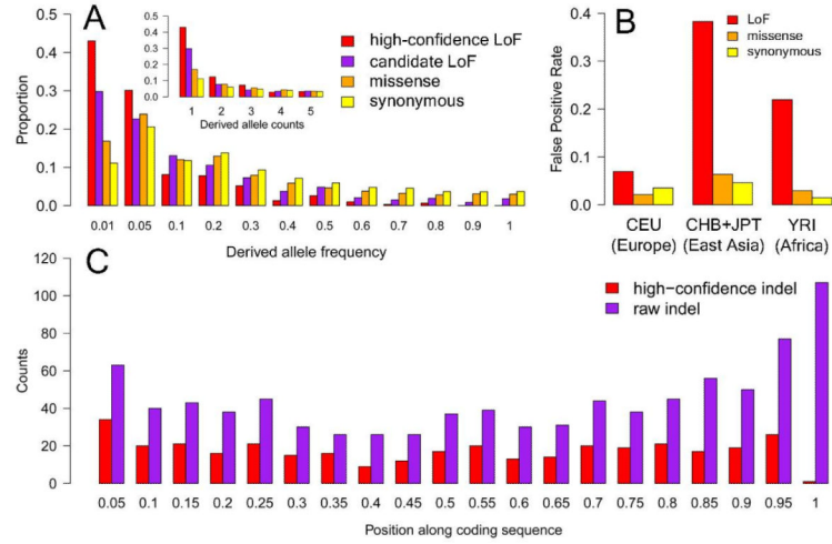
Figure 1. A. Derived allele frequency distribution in the CEU population for raw and high-confidence LoF variants, compared to missense and synonymous coding variants. Inset, distribution of the proportion of SNVs in each class at low allele counts (1-5). B. False positive rates (based on independent array genotyping) for LoF variants filtered for annotation artifacts and frequency-matched missense and synonymous SNVs. C. Distribution of frameshift indels along the coding region of affected genes, before and after filtering (a similar pattern is also seen for nonsense SNVs; data not shown).
