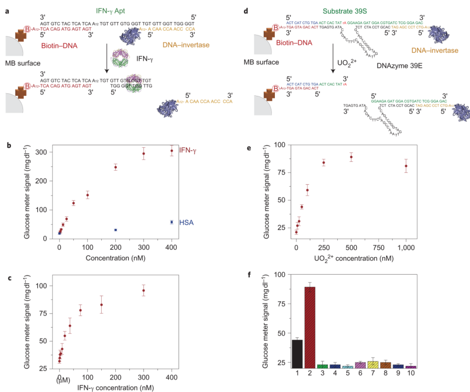
Figure 3. Design and performance of IFN- \gamma and UO 2 2+ detections using a PGM. a , IFN- \gamma -mediated release of immobilized DNA-invertase conjugates. b , IFN- \gamma detection in buffer using the PGM. c , IFN- \gamma detection in 20% human serum samples using the PGM. d , UO 2 2+ -mediated release of immobilized DNA-invertase conjugates. e , UO 2 2+ detection using the PGM. f , Selectivity of UO 2 2+ detection using the PGM: (1) 50 nM UO 2 2+ ; (2) 1 \mu M UO 2 2+ ; (3) 1 \mu M Pb 2+ ; (4) 1 \mu M Cd 2+ ; (5) 100 \mu M Ca 2+ /Mg 2+ ; (6) 1 \mu M Zn 2+ /Cu 2+ ; (7) 1 \mu M Co 2+ /Ni 2+ ; (8) 1 \mu M VO + ; (9) 1 \mu M Th 4+ ; (10) no metal ion. All error bars were obtained through the detection of three parallel samples.
