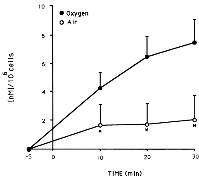
Figure 3. Generation of DMPO adducts by endothelial cell suspensions exposed to 100% oxygen (●, n = 12 ) or air (○, n = 12 ) for 30 min. DMPO (50 mM) was added 5 min before transferring the cells to an EPR flat cell at time 0 when the EPR measurements were begun. Brackets indicate \pm 1 SE; * P < 0.05 air compared to oxygen.
