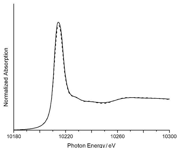
Figure 5. The tungsten L_3 edge XANES spectra of SAB (straight line) and bulk phosphotungstic acid (dotted line), indicating retention of the Keggin structure after immobilization.
