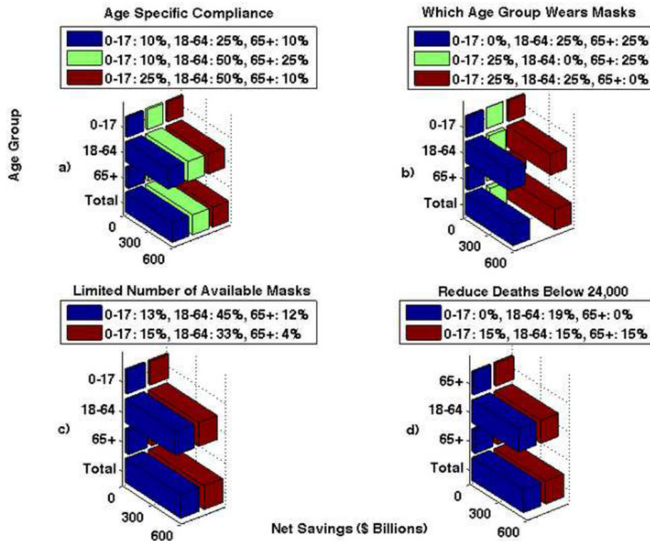
Figure 7. Net savings when the population wears N95 respirators that are 20% effective in reducing both infectivity and susceptibility, with an \mathcal{R}_{unc}^{avg}=1.3
