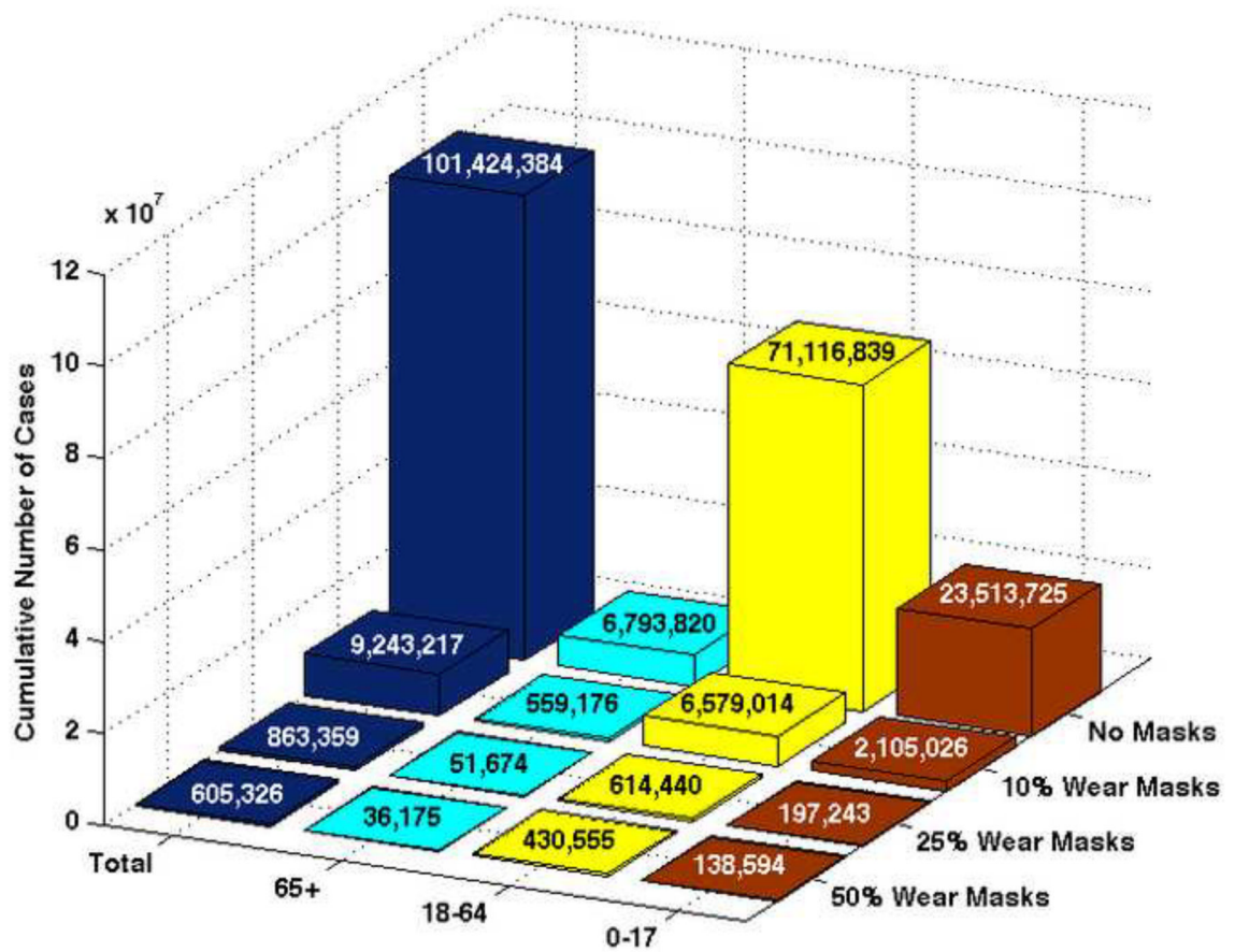
Figure 3. Cumulative number of pandemic (H1N1) 2009 cases when R_{unc}^{avg} = 1.25 and the N95 respirator is 20% effective in reducing both infectivity and susceptibility Three cases are shown when 10%, 25% and 50% of the total population wears masks.
