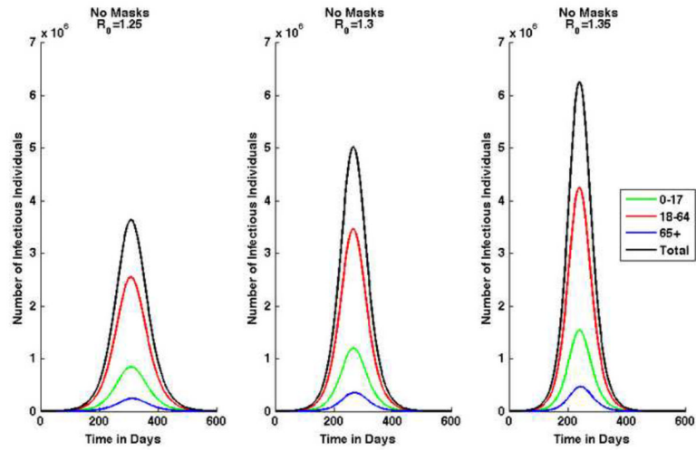
Figure 2. Epidemic curves by age group and combined total for pandemic (H1N1) 2009 when there are no masks worn
