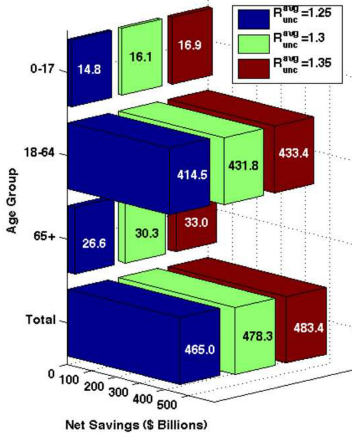
Figure 6. Net savings when 10% of the population is wearing N95 respirators and they are 20% effective in reducing both susceptibility and infectivity Three different pandemic severity scenarios are shown. The greatest net savings for the length of the pandemic are seen when the adult (18–64) age group wears masks.
