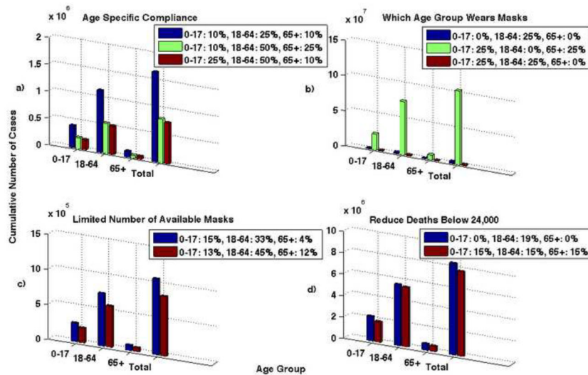
Figure 5. The number of cumulative cases for R_{unc}^{avg}=1.3 when N95 respirators are 20% effective in reducing both susceptibility and infectivity Part a shows the results for age specific compliance. Three different scenarios are shown: 1) 10% of children, 25% of adults, and 10% of seniors wear masks (blue bar), 2) 10% of children, 50% of adults, and 25% of seniors wear masks (green bar), 3) 25% of children, 50% of adults, and 10% of seniors wear masks (red bar). Note that the compliance rates of the children and seniors do not appear to decrease the disease spread, but the compliance rates of adults greatly reduces the number of cases. If only 25% of adults comply compared to 50% the number of cases nearly doubles. Part b shows the results when one group is not wearing masks and 25% of the other two remaining groups wearing masks. Note that if children or seniors do not wear masks the results are very similar, however, there is a large increase in the number of cases if adults do not wear masks. Part c shows the results when there is a limited number of masks available. The blue bar shows the number of cases if there are 75,500,000 masks available and the red bar shows if there are 100,000,000 masks available. Note that the goal in distributing the masks is to reduce the total number of deaths. Part d shows the results when the objective is to reduce the number of deaths below 24,000. The blue bars represent when 19% of adults wear N95 respirators and 0% of children and seniors wear them. The red bars represent when 15% of all age groups wear masks. Note that the number of cumulative cases is lower when 15% of the entire population; while it is important for the adult age group to wear masks, better results are seen when all age groups comply.
