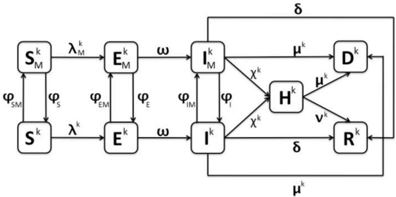
Figure 1. Schematic relationship between mask wearing and non-mask wearing individuals for pandemic (H1N1) 2009
