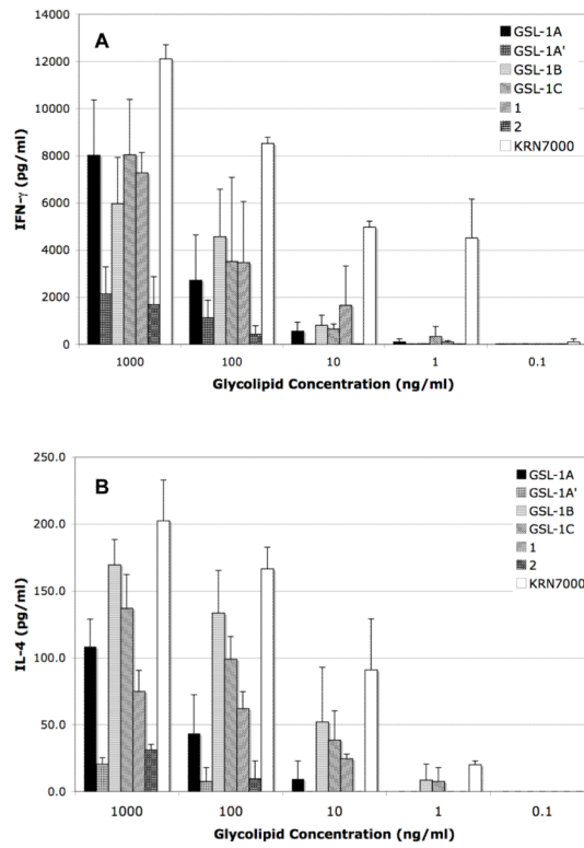
Figure 3. Cytokine production by splenocytes in response to the indicated glycolipids.
