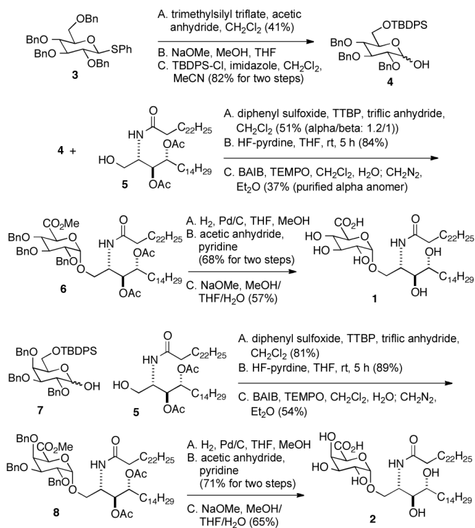
Scheme 1. Synthesis of glycolipids 1 and 2 .
