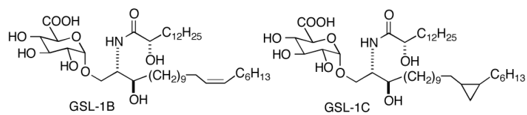
Figure 2. Structures of GSL-1B and GSL-1C .
