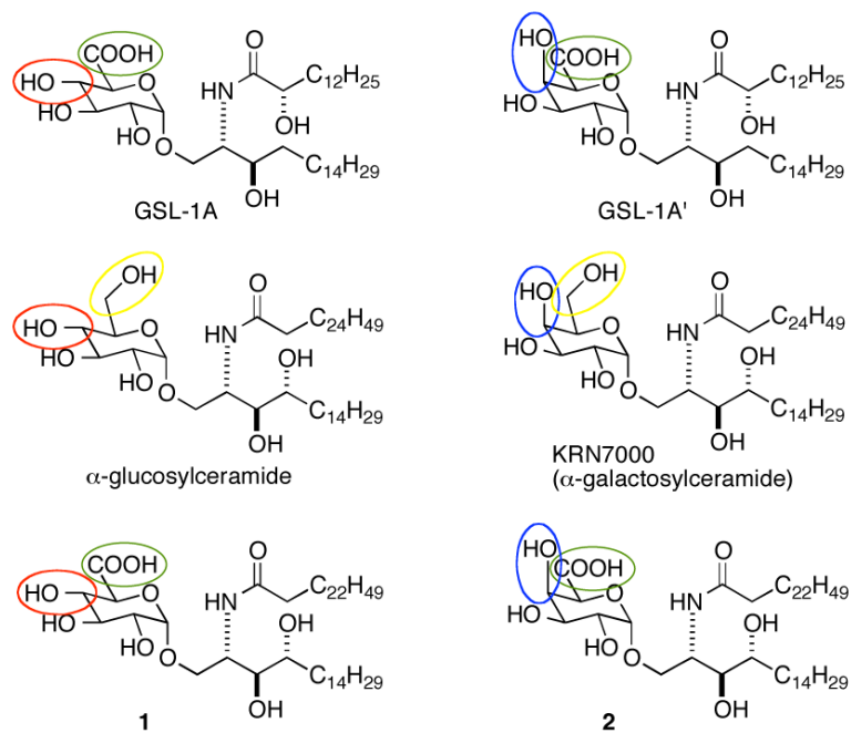
Figure 1. Structures of glycolipids from Sphingomonas (GSL-1A and GSL-1A'), NKT cell agonists α-glucosylceramide, KRN7000 and glycolipids 1 and 2.
