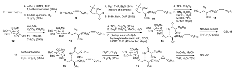
Scheme 2. Synthesis of GSL-1B and GSL-1C.
