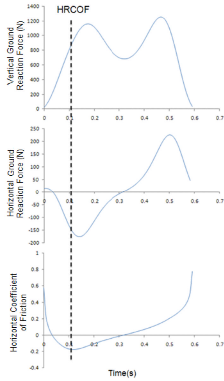
Figure 2. Horizontal coefficient of friction and its corresponding ground reaction force profiles
