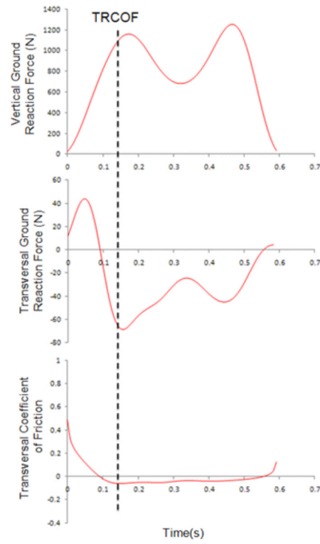
Figure 3. Transversal coefficient of friction and its corresponding ground reaction force profile
