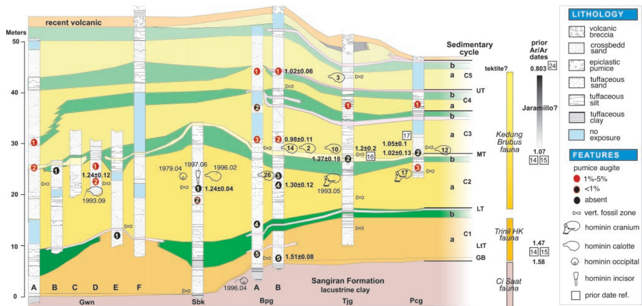
Fig. 2. Bapang Formation tephrostratigraphy. Sedimentary cycles: orange/yellow, a-facies; green, b-facies. Shading indicates the pattern of sediment fining from bottom to top. Numbered ovals mark epiclastic pumice sites sampled for augite content, hornblende color, and ^{40}\text{Ar}/^{39}\text{Ar} age analysis. From left to right, sections run north to south for a total of 4 km (no horizontal scale). The Grogolwetan and Bapang localities have lettered multiple sections. Pumice with hornblende ^{40}\text{Ar}/^{39}\text{Ar} ages \leq 1.1 Ma has 1–5 vol. % augite phenocrysts. Pcg-2, the exception (no augite), has an age of 1.02 \pm 0.13 Ma. Pumice with hornblende ^{40}\text{Ar}/^{39}\text{Ar} ages \geq 1.25 Ma lacks augite. Pumice from Gwn D-2 ( 1.24 \pm 0.12 Ma) has < 1\% augite microphenocrysts. At Grogolwetan, C2a pumice lens Gwn D-2 lies 50 cm above the cranium findspot. At Sendangbusik, C2a pumice lens Sbk-1 is in direct association with an incisor, a calotte, and two large occipital-parietal fragments, representing three individuals. The isotope correlation age ( 1.24 \pm 0.04 Ma) is shown for Sbk-1. At Bapang, B-1 represents UT (C4b), the only fine-grained tephra to give a reliable ^{40}\text{Ar}/^{39}\text{Ar} age ( 1.02 \pm 0.06 Ma). The C3a B-2 plateau age ( 0.98 \pm 0.11 Ma) is statistically indistinguishable from the UT age. C2a pumice at B-4 correlates stratigraphically with calotte S26. C1a pumice lens B-5 lies 130 cm above the Bapang/Sangiran contact. At Pucung, pumice lens Pcg-2 lies in association with a C3a fossil concentration.
