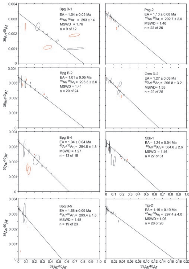
Fig. 4. Isotope correlation diagrams for hornblende isotopic results. Plots show combination of all data from each set of replicate analyses. Data shown in red are statistical outliers to the regression line as determined by the elimination methods of Deino and Potts (12).
