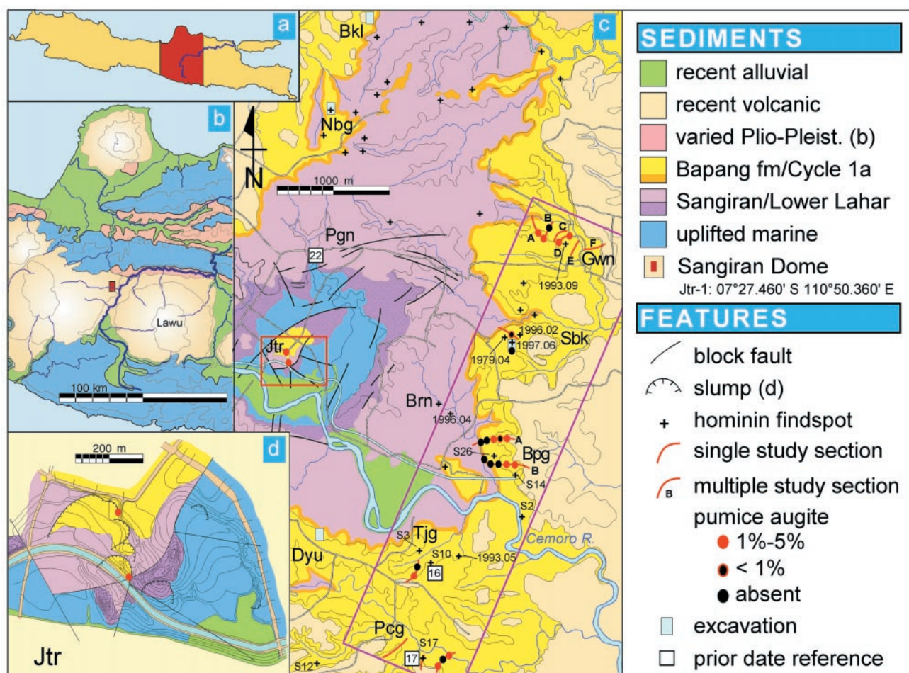
Fig. 1. (a) Java, Republic of Indonesia. (b) Solo Basin. The basin is a segment of Jawa's east-west trending Central Depression, the current magmatic zone of the Indonesian volcanic island arc. Supplying the Sangiran dome's Bapang Formation sedimentary sequence were volcanic cones building east and west and marine carbonate-silicate highlands emerging north and south. (c) Sangiran Dome. Southeast quadrant box shows locations for study sections, pumice samples, hominin findspots, and previous dates. +, documented hominin findspot (28, 29). Labeled findspots are discussed in the text or presented in Fig. 2. "S" prefix represents old colloquial "Sangiran" numbers used for fossils found into the mid 1970s. More recent findspots carry year and month of discovery along with a village locality prefix: Bkl, Brangkal; Brn, Bukuran; Bpg, Bapang; Dyu, Dayu; Gwn, Grogolwetan; Jtr, Jokotingkir Hill; Nbg, Ngebung; Pcg, Pucung; Pgn, Pablengan; Sbk, Sendangbusik; Tjg, Tanjung. (d) Jokotingkir Hill (central dome box). The lower red oval represents the Jtr-1 canal level pumice lens sampled for ^{40}\text{Ar}/^{39}\text{Ar} hornblende age analysis within a slumped Bapang Formation sediment block (longitude and latitude in legend). The upper red oval marks a pumice lens at the top of this block sampled for augite content and hornblende color only. Hominin fossils S27 and S31 were recovered during canal excavations within 150 m west-northwest of Jtr-1.
