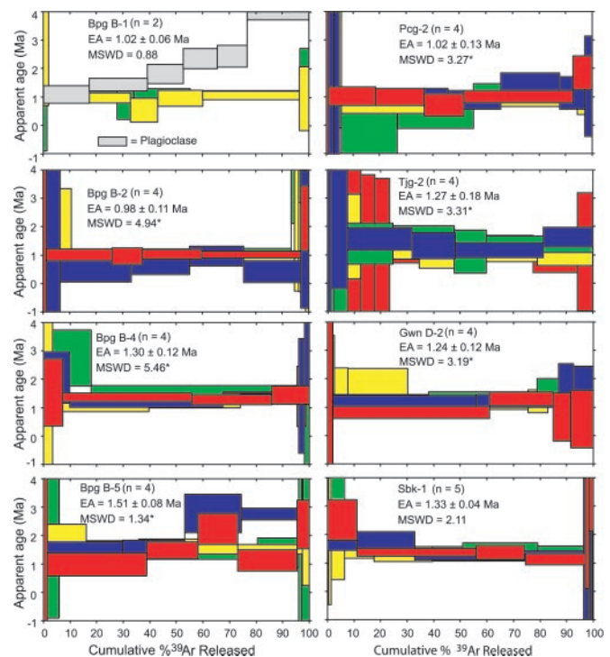
Fig. 3. ^{40}\text{Ar}/^{39}\text{Ar} age spectra diagrams for replicate (n) hornblende analyses. EA, Eruption Age. Overall, the replicate analyses are reproducible and have flat age spectra. Both plagioclase and hornblende separates were analyzed from site Bpg B-1. In contrast to the hornblende from this sample, the plagioclase yielded a highly discordant spectrum.
