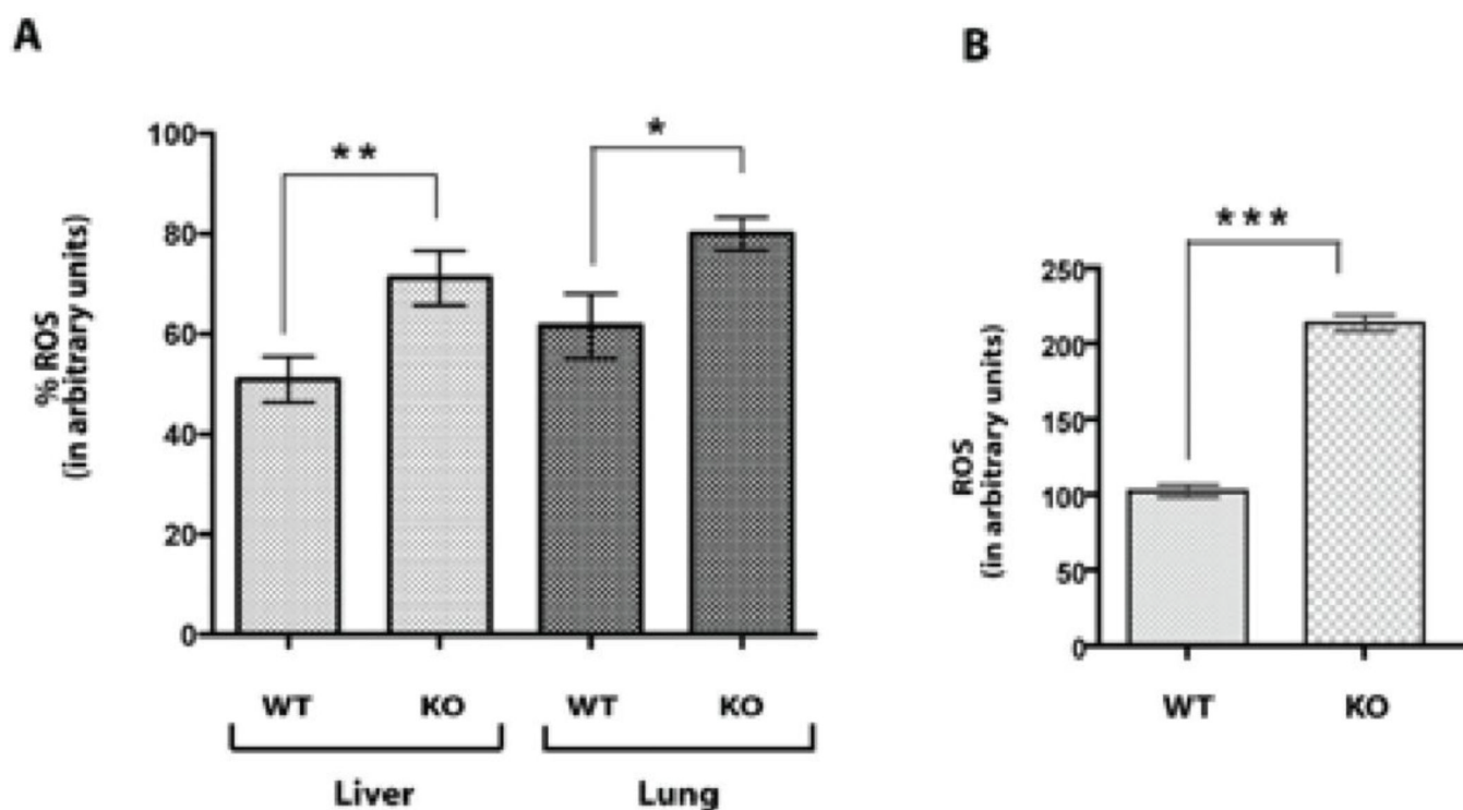
Figure 3. Sigma-1 receptor KO mice have higher oxidative stress
