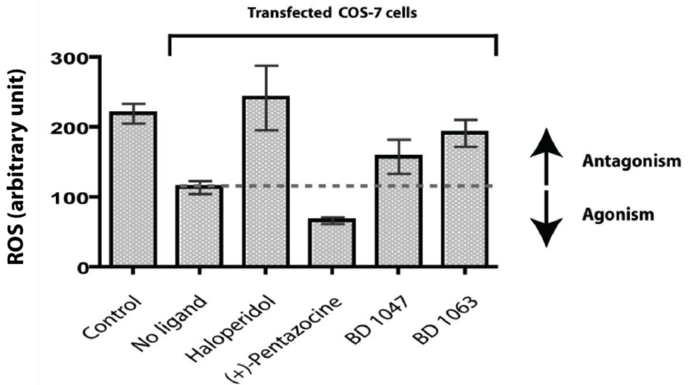
Figure 4. Sigma-1 receptor protects COS-7 cells from oxidative stress
