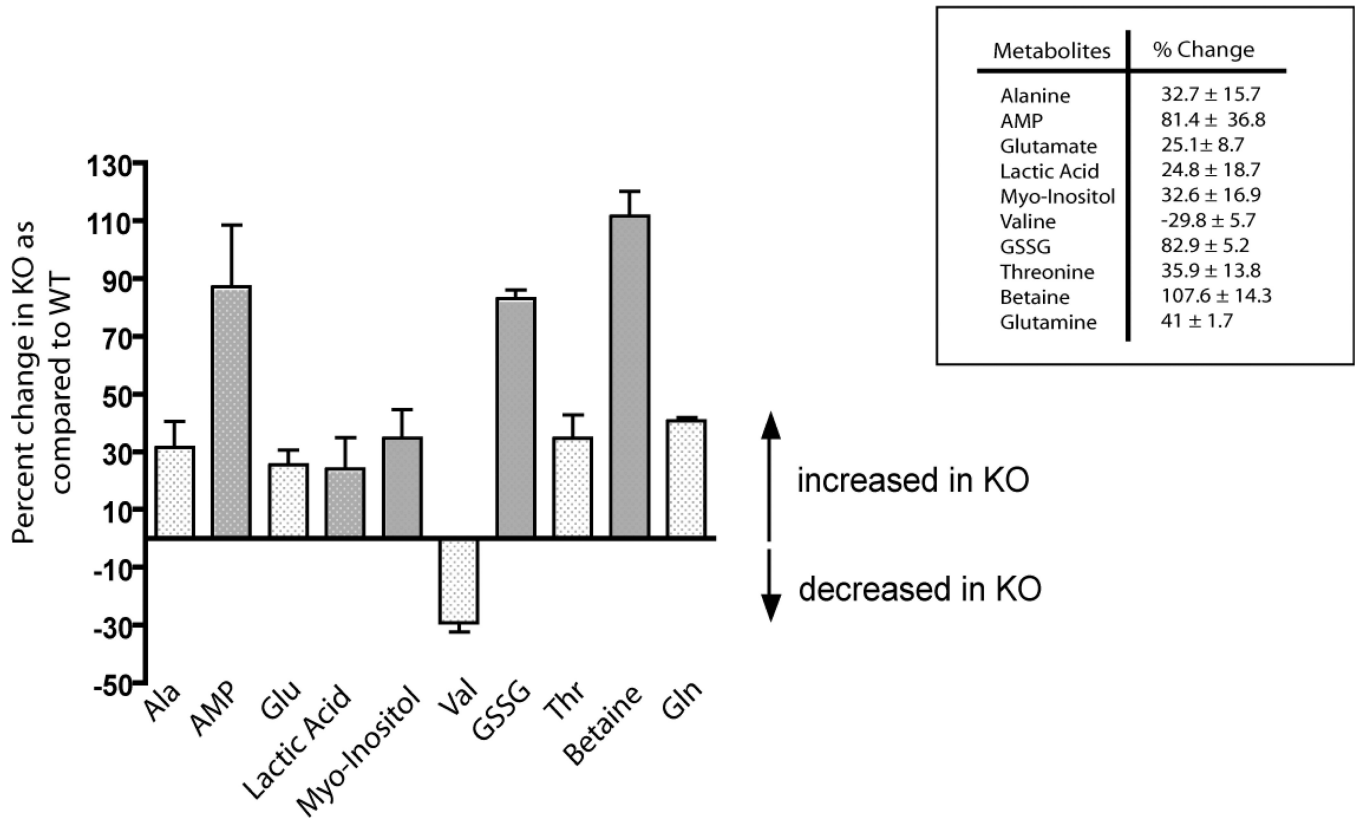
Figure 1. Changes in metabolites in the WT and sigma-1 receptor KO mouse livers. Higher levels of oxidized glutathione (GSSG) and glutamate in the KO livers indicate that the KO mice were under oxidative stress. Error bars represent mean \pm S.E.M. from different experiments (n = 6).
