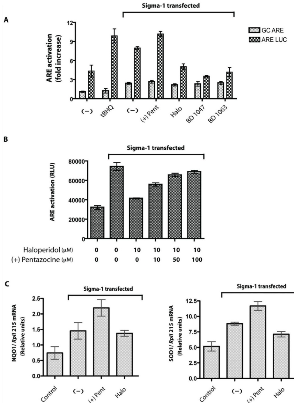
Figure 5. Sigma-1 receptor activates 'Antioxidant Response Elements' (ARE)
