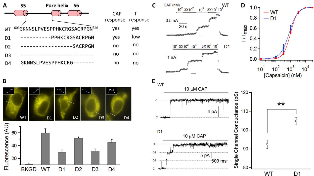
Figure 1. TRPV1 turret deletion mutants. (A) Diagram illustrating turret deletion mutants and their responses to 10 \mu\text{M} capsaicin and heat (50°C or higher). Dashes indicate deletion of amino acids. (B) Cell images demonstrating similar cellular expression patterns between WT TRPV1 and deletion mutants. Fluorescence intensity profile along the indicated line is shown in inset. An intensity peak is visible at the location of plasma membrane. The bottom panel shows quantitation of fluorescence intensity at the plasma membrane. (C) Capsaicin-induced currents from WT (top) and D1 mutant channels (bottom). (D) Dose-dependent activation of WT and D1 by capsaicin. Curves represent fits of a Hill equation to the averaged datasets. The EC 50 and slope factor values are: 0.98 \mu\text{M} and 1.9 ( n = 3 ) for WT, and 0.80 \mu\text{M} and 1.5 ( n = 4 ) for D1. (E) Single-channel trace (left) and conductance (right) of WT and D1 in response to 10 \mu\text{M} capsaicin. Representative traces of four similar recordings for WT and five for D1. **, P < 0.01 .
