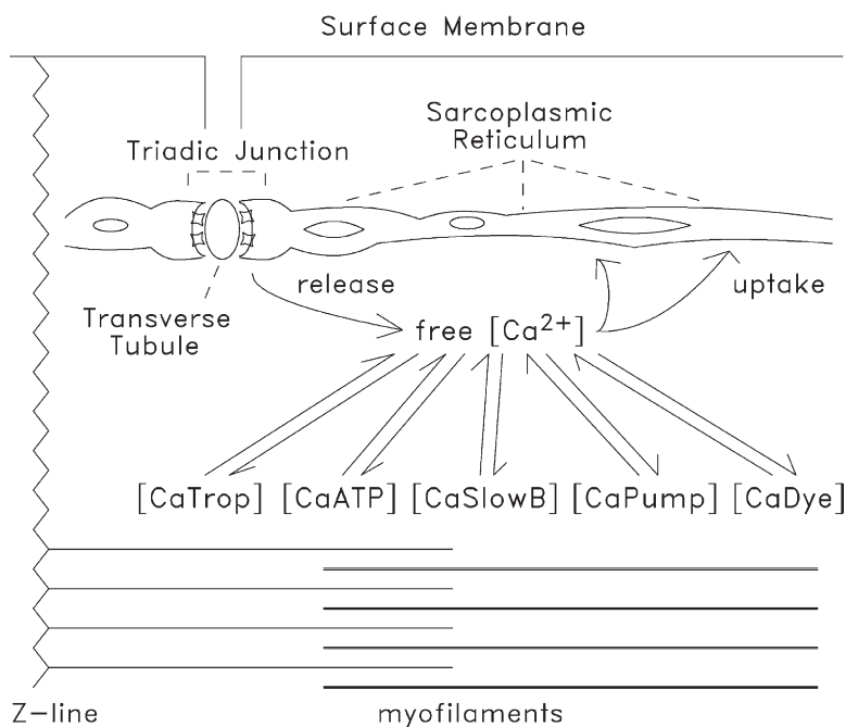
Figure 1. Schematic of intra-sarcomeric Ca 2+ movements during excitation–contraction coupling in mammalian skeletal muscle fibers. Depolarization of the transverse tubular membranes initiates Ca 2+ release from the SR at the triadic junctions. The rise in myoplasmic free [Ca 2+ ] drives Ca 2+ complexation with the major myoplasmic Ca 2+ buffers: (a) troponin (located on the thin filaments); (b) ATP; (c) other proteins (“SlowB”) such as parvalbumin, which, in rodent fibers, is found at a large concentration in fast-twitch glycolytic fibers but not in slow-twitch fibers (Table 2); (d) Ca 2+ pump molecules (located in the SR membranes); and (e) the Ca 2+ indicator dye (which can be introduced experimentally to monitor Δ[Ca 2+ ]).
