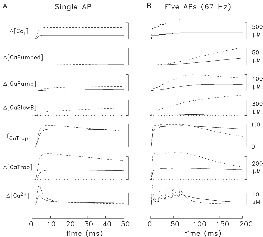
Figure 4. Comparison of \text{Ca}^{2+} movements elicited by APs in slow-twitch and fast-twitch fibers (16°C). (A). Simulated \text{Ca}^{2+} movements in slow-twitch and fast-twitch fibers (continuous and dashed traces, respectively) in response to a single AP initiated at zero time. f_{\text{CaTrop}} , the fractional occupancy of the troponin regulatory sites with \text{Ca}^{2+} , includes the resting occupancy (0.071 in slow-twitch fibers and 0.004 in fast-twitch fibers) plus the change in occupancy during activity. See text for definitions of the other traces. \Delta[\text{CaT}] is the sum of the five lower traces, excluding f_{\text{CaTrop}} , plus \Delta[\text{CaATP}] and \Delta[\text{CaDye}] (the change in the concentration of \text{Ca}^{2+} bound to the indicator). \Delta[\text{CaATP}] is approximately equal to 2.2 times \Delta[\text{Ca}^{2+}] in slow-twitch fibers and 3.4 times \Delta[\text{Ca}^{2+}] in fast-twitch fibers. \Delta[\text{CaDye}] is relatively small ( = \Delta f_{\text{CaD}} \times [\text{Dye}_T] , where [\text{Dye}_T] , the total indicator concentration in myoplasm, is 100 \mu\text{M} ). The units of all traces except f_{\text{CaTrop}} are spatially averaged concentrations referred to the myoplasmic water volume. (B). As in A, but for five APs at 67 Hz.
