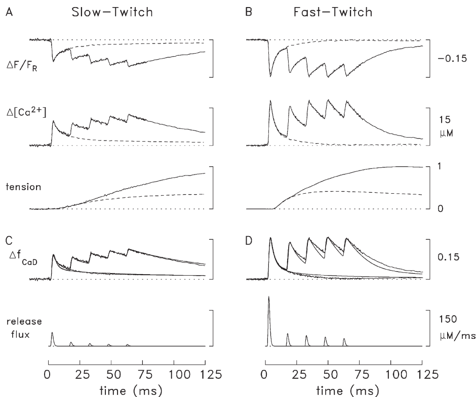
Figure 2. Ca 2+ -related fluorescence signals and tension responses in slow-twitch and fast-twitch mouse fibers stimulated by APs (16°C). (A and B) Bundles of fibers from soleus muscles (A) and EDL muscles (B) of adult mice, age 7–14 wk, were isolated by dissection, and one fiber within the bundle was micro-injected with either furaptra or mag-fluo-4. \Delta F/F_R and tension responses were recorded in response to external stimuli that elicited either one AP (dashed traces) or five APs at 67 Hz (continuous traces); the responses to both types of stimulation are shown superimposed. All traces represent averaged responses from several experiments in which movement artifacts in the \Delta F/F_R traces were small. All fast-twitch experiments were performed on fibers injected with furaptra (seven fibers in the measurements with a single AP, four in the measurements with five APs); the fast-twitch fibers are from a region of the EDL muscle thought to be rich in parvalbumin (see Baylor and Hollingworth, 2011). The slow-twitch experiments with a
