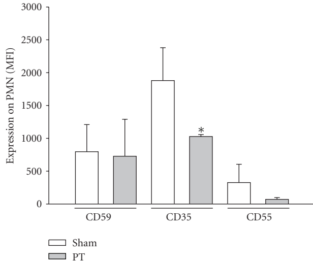
FIGURE 5: Complement regulatory response after trauma, CReg Expression (MFI) CD59, CD35 and CD55 on neutrophils (PMNs) in Sham- and PT rats 4 hrs after trauma. All data are presented as mean \pm SD. * P < 0.05 . n = 6 –10 rats/group.
