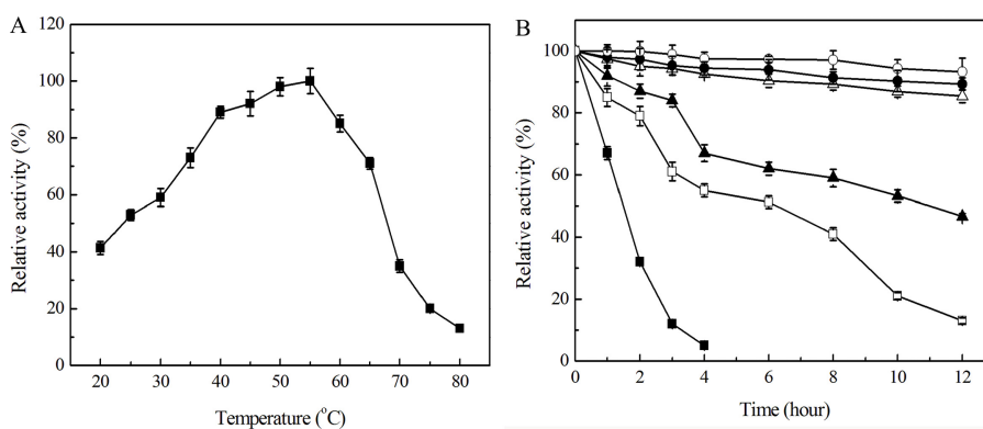
Figure 5 Effect of temperature on activity (A) and stability (B) of recombinant Sys410. The purified enzyme was preincubated at 35°C (○), 40°C (●), 45°C (▲), 50°C (△), 55°C (□) for 12 hours.
