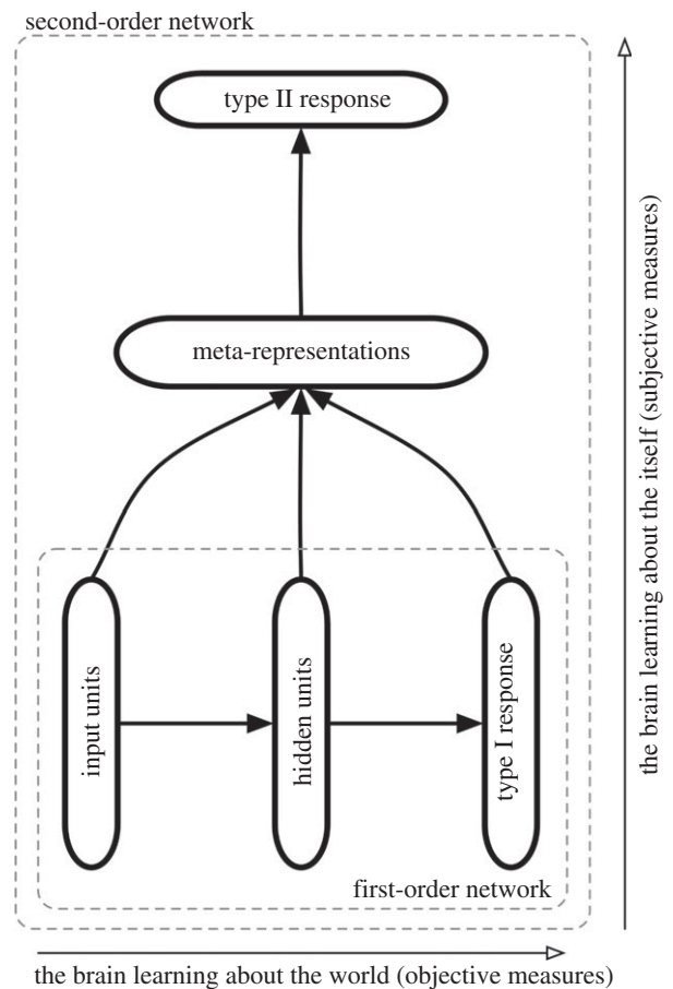
Figure 1. General architecture of a metacognitive network. A first-order network, consisting, for instance, of a simple three-layer backpropagation network, is trained to perform a simple classification task and thus contains knowledge that links inputs to outputs in such a way that the network can produce type I responses. This entire first-order network then constitutes the input to a second-order network, the task of which consists of re-describing the activity of the first-order network in some way. Here, the task that this second-order network is trained to perform is to issue type II responses, that is, judgements about the extent to which the first-order network has performed its task correctly. One can think of the first-order network as instantiating cases where the brain learns about the world and of the second-order network as instantiating cases where the brain learns about itself.
