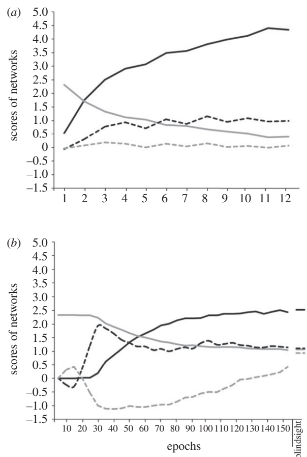
Figure 3. SDT analyses of the model’s performance. The chart in (a) (type I and type II scores) reflects both objective and subjective measures in the AGL simulation; the chart in (b) (type I and type II scores) reflects both objective and subjective measures in the blindsight simulation. (Data points for blindsight test type I d' and type II c overlap.) Solid black line, type I d' ; dashed black line, type II d' ; solid grey line, type I c ; dashed grey line, type II c .
