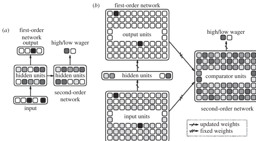
Figure 2. (a) Network architecture for the Iowa Gambling Task simulation (see [2], simulation 3). The network consists of a first-order feedforward backpropagator, of which the hidden units feed forward into a set of second-order hidden units, which in turn feed forward into two wagering units. (b) Network architecture for the Blindsight and artificial grammar learning (AGL) simulations (see [2], simulations 1 and 2). The network consists of a first-order feedforward backpropagation autoassociator, of which the input and output units are connected through fixed weights to a second-order comparator, which in turn feeds forward into two wagering units.
