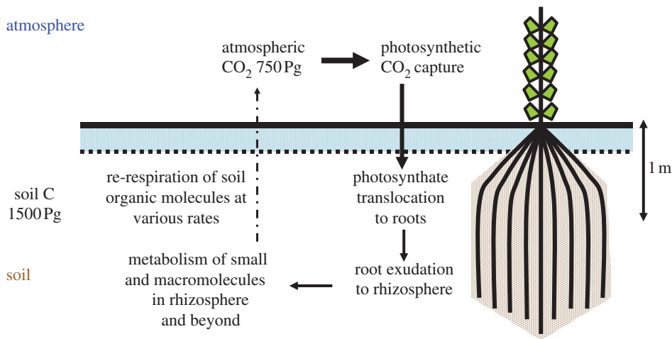
Figure 2. High-level analysis of the major processes involved in soil carbon sequestration for photosynthetically fixed CO 2 .
