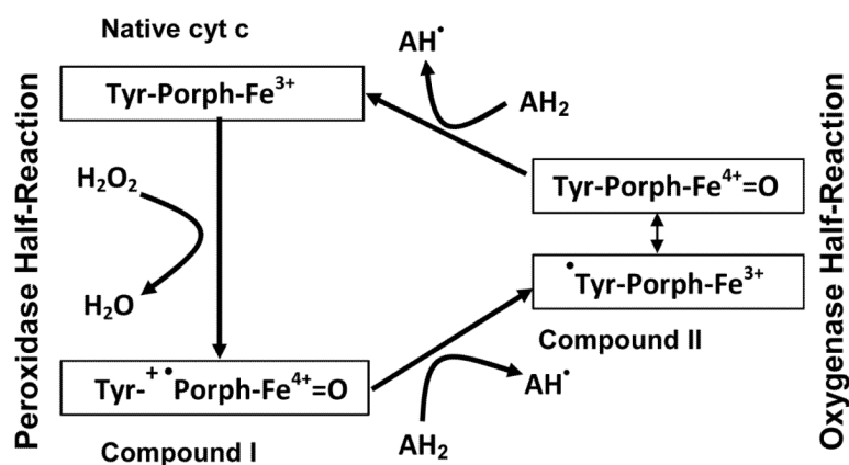
Figure 1. General scheme of peroxidase cycle of cyt c
