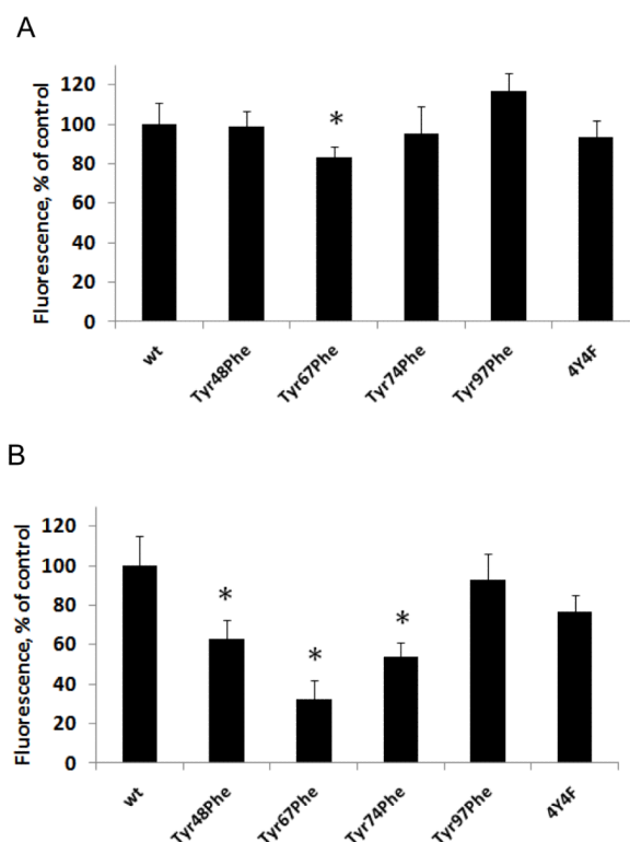
Figure 6. Peroxidase activity of complexes of cyt c with TOCL (wild type and mutated cyt c) measured by the fluorescence of resorufin (an Amplex Red oxidation product) Incubation conditions: concentration of cyt c was 1 \mu M, TOCL/cyt c ratio was 20:1, 50 \mu M Amplex Red and 25 \mu M H 2 O 2 . Buffer-20 mM HEPES (pH 7.4), 100 \mu M DTPA (A), or PBS, 100 \mu M DTPA (B), *p<0.01 vs. wild-type cyt c.
