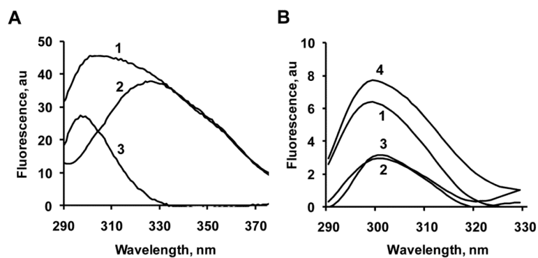
Figure 5. Fluorescence spectra of wild type and mutant forms of horse heart cyt c. Assessments of contribution of different Tyr residues in total tyrosine fluorescence of cyt c
