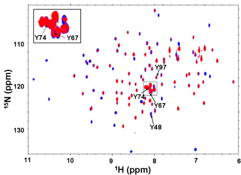
Figure 4. NMR spectra of cyt c
