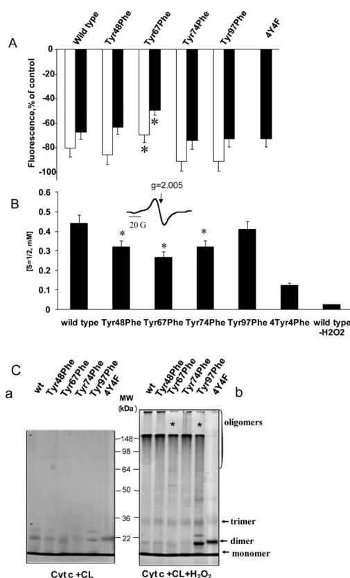
Figure 7. H 2 O 2 -dependent changes in Tyr and Trp fluorescence, production of protein-derived radicals and oligomerization of wild type and mutated forms of cyt c
