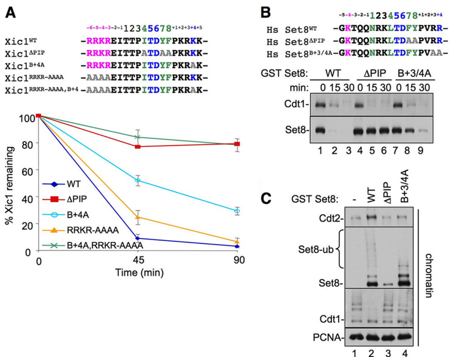
FIGURE 2. The B+4 residue can be partially compensated for by residues upstream of the PIP box in Xic1 and Set8. In A : Top, sequence comparison of Xic1 PIP degron with upstream basic residues and the various mutants examined. Bottom, graph showing the percentage of in vitro translated 35 S-labeled Xic1 remaining after it was added to HSS in the presence of 5 ng/μl MMS-damaged plasmid. Reactions were stopped at the indicated time points, and the amount of Xic1 remaining was quantified by autoradiography. Results from three independent experiments were averaged and graphed. Bars represent the standard error of the mean. In B : Top, sequence alignment of Set8 PIP degron with upstream residues and the various mutants examined. Bottom, HSS was supplemented with 5 ng/μl MMS plasmid and 50 nM human Set8 WT , Set8 ΔPIP , or Set8 B+3/4A . At the indicated times, samples were blotted for endogenous Cdt1 or Set8. C, HSS was supplemented with immobilized 1-kb MMS DNA and 2 mg/ml methyl ubiquitin. Buffer and 50 nM Set8 WT , Set8 ΔPIP , or Set8 B+3/4A was also added, and after 10 min, chromatin was recovered from the extract and washed, and the indicated proteins were visualized by Western blotting.
