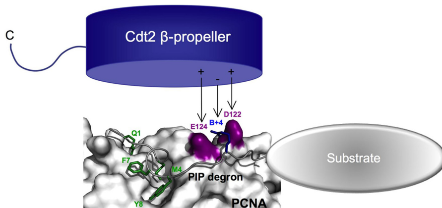
FIGURE 7. Putative model of CRL4 Cdt2 recruitment to the PCNA-substrate complex. Substrate-dependent recruitment of CRL4 Cdt2 to PCNA DNA requires residues in the PIP degnon (B+4), as well as PCNA Asp-122. PCNA Glu-124 also contributes to CRL4 Cdt2 recruitment but is not essential. We speculate charged residues in Cdt2 make direct contacts with B+4, Asp-122, and Glu-124.
