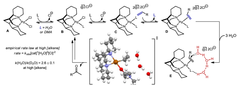
Figure 5. Proposed mechanism of the direct \text{O}_2 -coupled Wacker oxidation using \text{Pd}[(-)\text{-sparteine}]\text{Cl}_2
