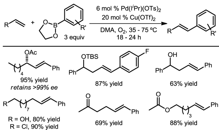
Figure 11. Selected scope of electronically non-biased alkenes as substrates in catalyst controlled oxidative Heck reactions.
