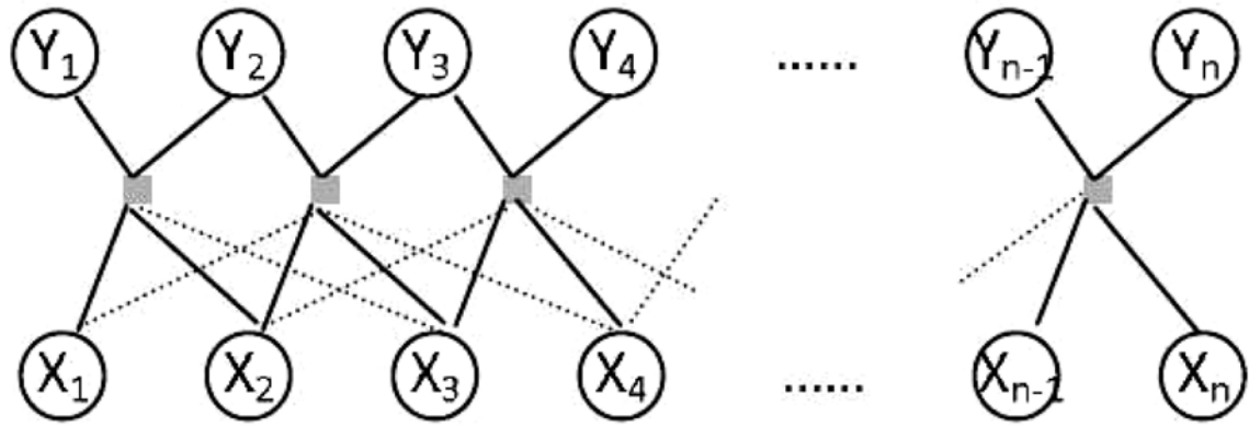
Fig. 2. A linear chain conditional random field model for array CGH data.
