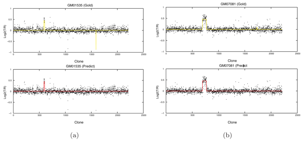
Fig. 3. Predicted breakpoints by CRF-CNV (bottom) vs. true breakpoints (up) on two cell lines GM01535 (a) and GM07081 (b).
