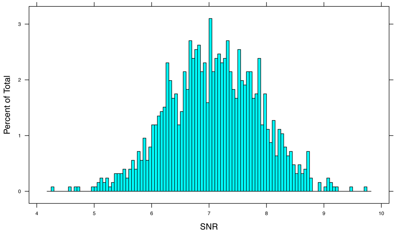
Figure 1. Signal to noise ratio for the HapMap phase 3 data. Signal to noise ratios below 5 can indicate problems with data quality.
