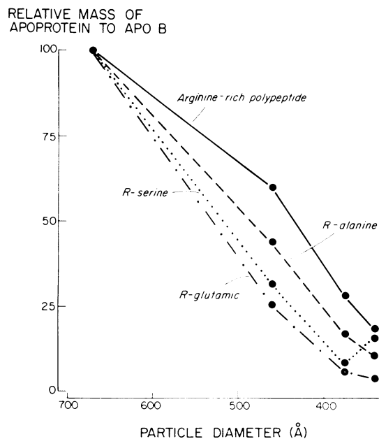
FIGURE 6 Ratio of four apoproteins relative to apoB as a function of particle size. For comparability, the ratio of each apoprotein to apoB in each particle fraction is expressed as a percentage of the ratio of that individual apoprotein to apoB in the largest particles (mean diameter, 671 Å) taken as 100 (ordinate). The abscissa gives the mean particle diameter of the fraction. Each point is the mean of duplicate determinations.
