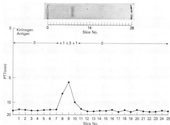
FIGURE 10 Alkaline disc gel electrophoresis at pH 9.3 of 30 \mu\text{g} of high molecular weight kininogen (B4- \gamma ) obtained from Bio-Gel 0.5 m. A replicate disc gel was sliced and eluted, and this eluate was assayed for kininogen antigen by counterimmuno-electrophoresis and for its ability to correct the coagulation defect of Williams trait plasma.
