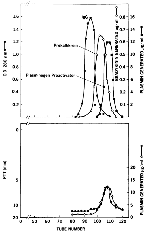
FIGURE 6 Sephadex G 150 gel filtration of the mixture of prekallikrein and plasminogen proactivator derived from the QAE Sephadex effluent (Fig. 5). Below is shown the ability of these fractions to correct the coagulation and fibrinolytic abnormalities of Williams trait plasma.
