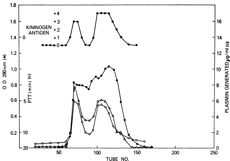
FIGURE 9 Sephadex G 150 gel filtration of the major peak of corrective activity eluted from SP Sephadex (Fig. 7). The column fractions of the major peak were assayed for kininogen antigen by counter-immunoelectrophoresis and for their ability to correct the coagulation and fibrinolytic abnormalities in Williams trait plasma.
