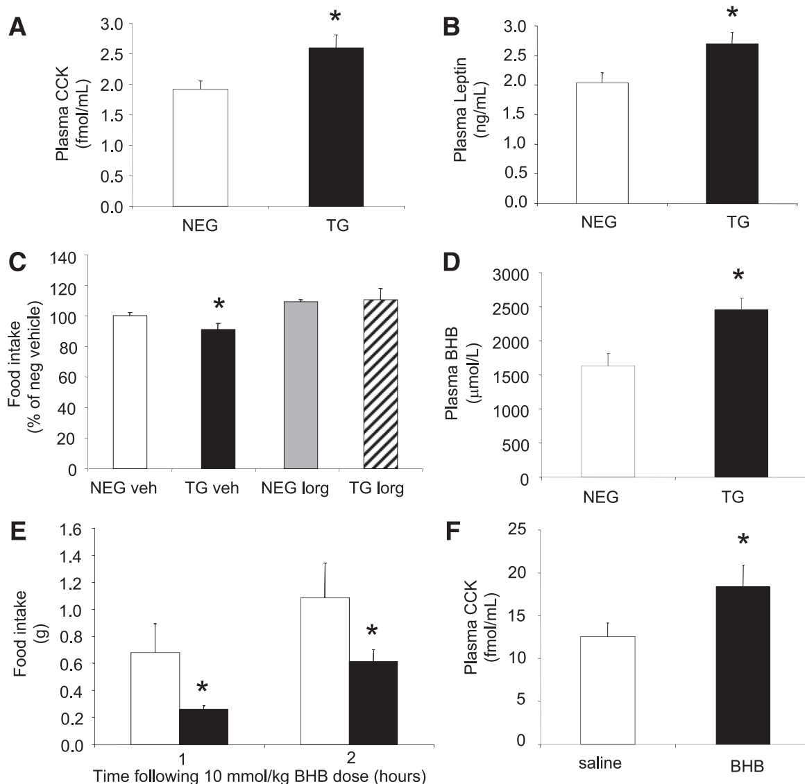
FIG. 5. Increased satiety hormones in livers of FBPase transgenic (TG) mice. Circulating CCK (A) and circulating leptin (B) levels in hemizygous TG (black bars) and negative (NEG, white bars) littermate mice ( n = 6 ). *P < 0.05 vs. NEG, one-way ANOVA. C: Food intake levels after CCK1 receptor antagonist (lorglumide [LORG], 300 \mu\text{g}/\text{kg} ) treatment ( n = 5 ). *P < 0.05 vs. all groups, one-way ANOVA. D: Circulating BHB concentrations in hemizygous TG (black) and NEG (white) littermate mice ( n = 8 ). *P < 0.05 vs. NEG, one-way ANOVA. Food intake levels at 1 and 2 h (E) and circulating CCK concentration at 1 h (F) after BHB (10 mmol/kg) administration to C57Bl/6J mice ( n = 16 ). *P < 0.05 vs. NEG, one-way ANOVA. All data expressed as mean \pm SEM.
