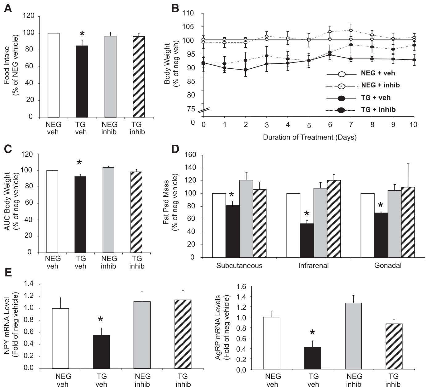
FIG. 4. Pharmacologic inhibition of FBPase in transgenic (TG) mice. Percentage daily food intake (A), body weight (B), AUC body weight (C), fat pad mass (D), and ARC neuropeptide mRNA levels (E) of FBPase inhibitor (INHIB)-treated (dashed line) and vehicle (VEH)-treated (bold line) hemizygous TG (black bars/circles) and negative (NEG, white bars/circles) littermate mice after 10 days of inhibitor (5 mg/kg) treatment ( n = 4 for each group). * P < 0.05 vs. all groups, one-way ANOVA. All data expressed as mean \pm SEM.
