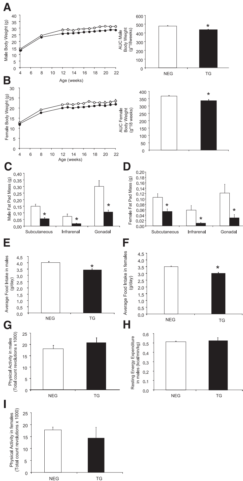
FIG. 1. Characterization of liver FBPase transgenic (TG) mice. Body weights of male negative (NEG, white circles ) and TG ( black circles ) mice from hemizygous breeding from age 4 weeks to 22 weeks (NEG: n = 11 and TG: n = 14 ; AUC *P < 0.001 vs. NEG, GLM ANOVA) (A) and female NEG ( white circles ) and TG ( black circles ) mice from hemizygous breeding from age 4 weeks to 22 weeks (NEG: n = 13 and TG: n = 10 ; AUC *P < 0.005 vs. NEG, GLM ANOVA) (B). Fat pad mass of male hemizygous TG mice ( black bars ) compared with their NEG ( white bars ) littermates (NEG: n = 14 and TG n = 9 ; *P < 0.02 vs. NEG, one-way ANOVA) (C) and female hemizygous TG mice ( black bars ) compared with their NEG ( white bars ) littermates at age 24 weeks (NEG: n = 11 and TG: n = 6 ; *P < 0.05 vs. NEG, one-way ANOVA) (D). Average daily food intake of male hemizygous TG mice ( black bars ) compared with NEG ( white bars ) littermates (NEG: n = 21 and TG: n = 14 ; *P < 0.0001 vs. NEG GLM ANOVA) (E) and of female hemizygous TG mice ( black bars ) compared with NEG ( white bars ) littermates (NEG: n = 18 and TG: n = 10 ; *P < 0.05 vs. NEG, GLM ANOVA) (F). Physical activity (NEG: n = 7 and TG: n = 5 ) (G) and resting energy expenditure ( n = 4 for each group) (H) in male hemizygous transgenic mice ( black bars ) compared with negative ( white bars ) littermates. I: Physical activity measurements of female hemizygous TG ( black bars ) compared with NEG ( white bars ) littermates (NEG: n = 10 and TG: n = 4 ). All data expressed as mean \pm SEM.
