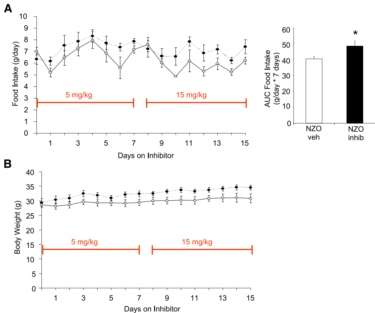
FIG. 7. Pharmacologic inhibition of FBPase in the NZO mouse. Food intake (absolute g/day) and AUC of food intake on 15 mg/kg inhibitor treatment over 7 days ( panel inset ) (A) and body weight (B) of NZO mice treated with FBPase inhibitor ( black circles ) or with vehicle ( white circles ) for 15 days ( n = 5 per group). * P < 0.05 vs. NZO vehicle-treated mice, GLM ANOVA. All data expressed as mean \pm SEM. (A high-quality color representation of this figure is available in the online issue.)
