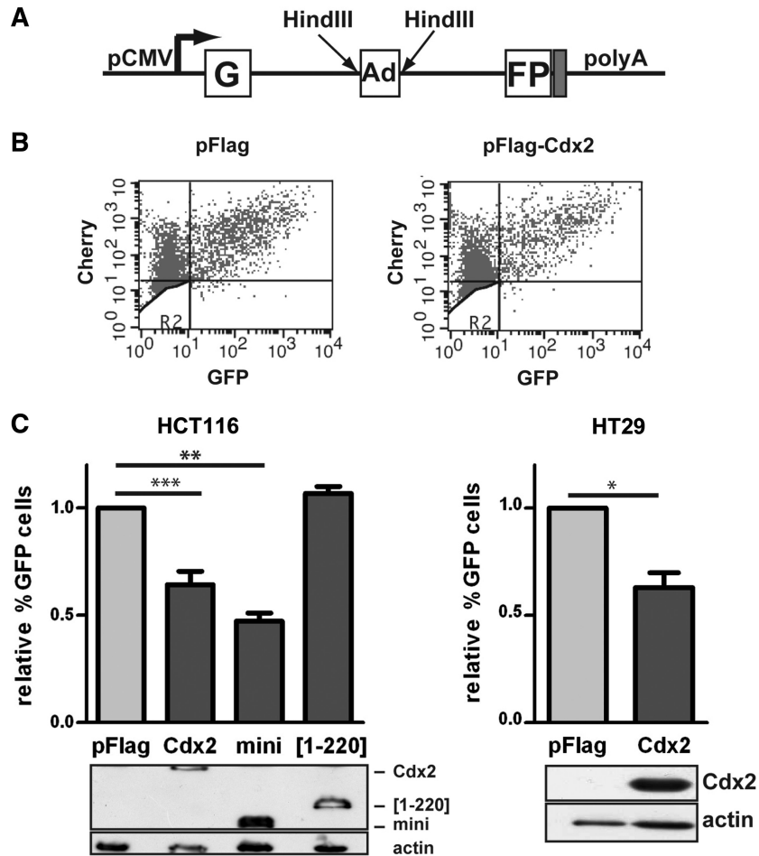
Figure 5. Cdx2 inhibits DNA repair in vivo in intestinal cells. (A) Schematic representation of the pEGFP-Pem1-Ad2 plasmid. G and FP corresponds to the 5' and 3' part of the GFP encoding cDNA. Ad corresponds to the adenoviral intron flanked by two HindIII sites. pCMV indicates the CMV promoter. (B) Example of green-versus-red fluorescent plots. The experiment was performed in HCT116 transfected with pFlag (left panel) or pFlag-Cdx2 (right panel). X axis: green fluorescence; Y axis: red fluorescence. (C) Cdx2 alters the in vivo DNA repair. Results represent the mean of at least four experiments performed in HCT116 (left panel) or HT29 (right panel) transfected with either pFlag, pFlag-Cdx2, pFlag-miniCdx2 or Cdx2[1-220] plasmids as indicated. The percentage of GFP and Cherry double positive cells in the Cherry positive cell population was set at 1 for pFlag and error bars represent SEM. Asterisk indicate a significant difference (** P < 0.01 ; * P < 0.05 ). Above, expression of Cdx2 and its mutants was checked by western blot on 10 \mu g of whole protein extracts using anti-Flag antibody. Actin was used as loading control.
