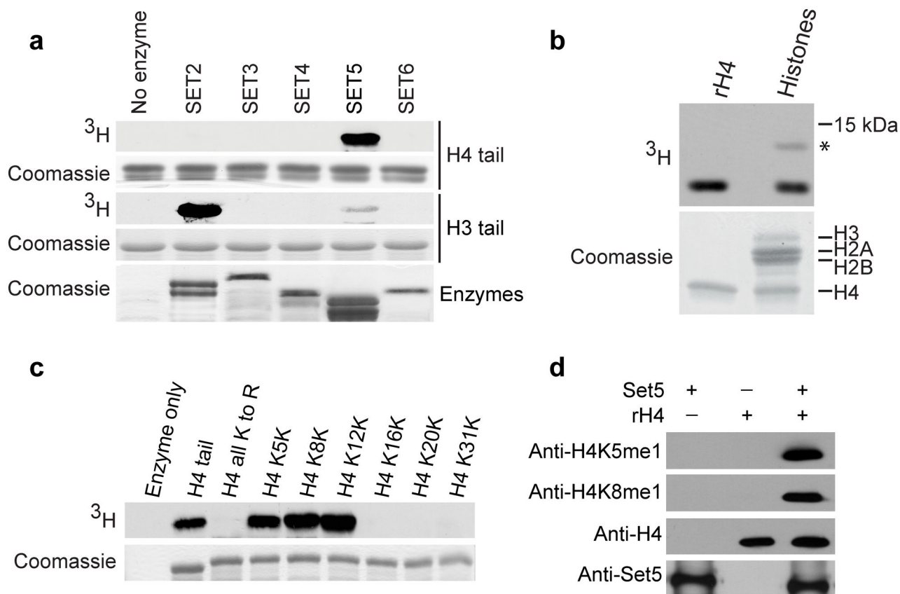
Figure 1. Identification of Set5 as an H4 methyltransferase. (a) Methylation assays with recombinant SET domain enzymes, H3 and H4 tails using ^3\text{H} -SAM as the methyl donor. Autoradiograph and Coomassie (loading control) are shown. (b) Set5 methylates recombinant H4 (rH4) and H4 from native histones purified from calf thymus (* indicates H2A). (c) Set5 methylates lysines 5, 8 and 12. Methylation assay on H4 tails with lysines mutated to arginine (all K to R) or single lysines maintained and all other lysines mutated to arginine. (d) Monomethylation of H4K5 and H4K8 on rH4. Immunoblots with the indicated antibodies are shown.
