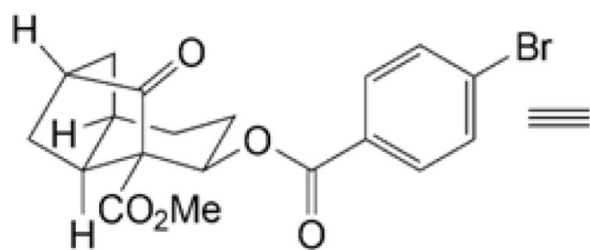
Figure 2. ORTEP representation of 22
