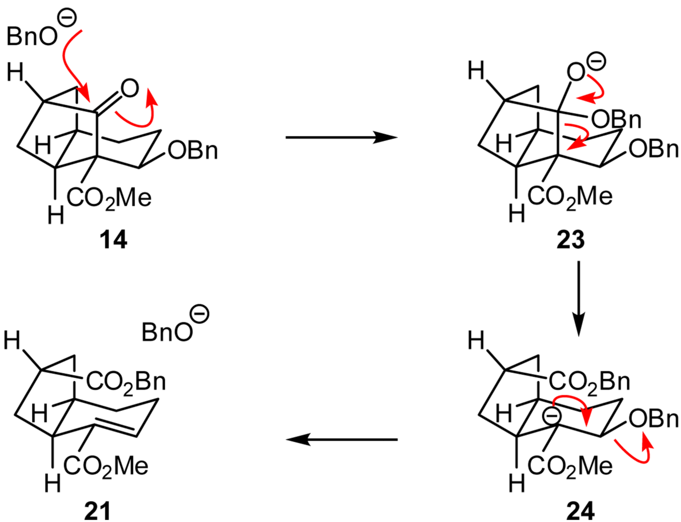
Scheme 5. Fragmentation pathway of 14
