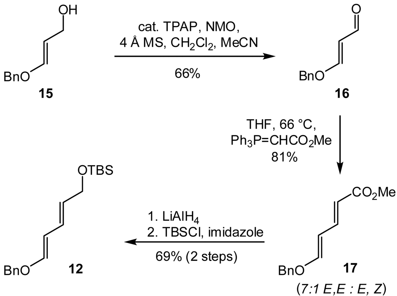
Scheme 3. Synthesis of diene 12
