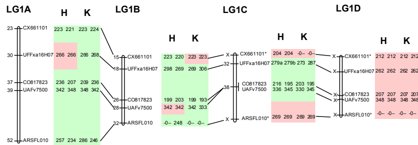
Figure 3 Linkage maps for the four homoeologous chromosome pairs of LG1 in the allo-octoploid strawberry. These maps are based on the five microsatellites that have been used to exemplify the MADCE approach for the assessment of allele doses and assignment of sub-genomes based on parent-specific allelic pairs. Positions (in cM) are shown on the left side of each linkage group (LG). Positions with an x instead of a value are homozygous in both parents and therefore cannot be used for determining map distances. A green background indicates heterozygosity, and a red background indicates homozygosity. H and K indicate the 'Holiday' and 'Korona' parents, respectively. * Allelic configurations are interchangeable between the related homoeologues. 0: inferred null allele.
