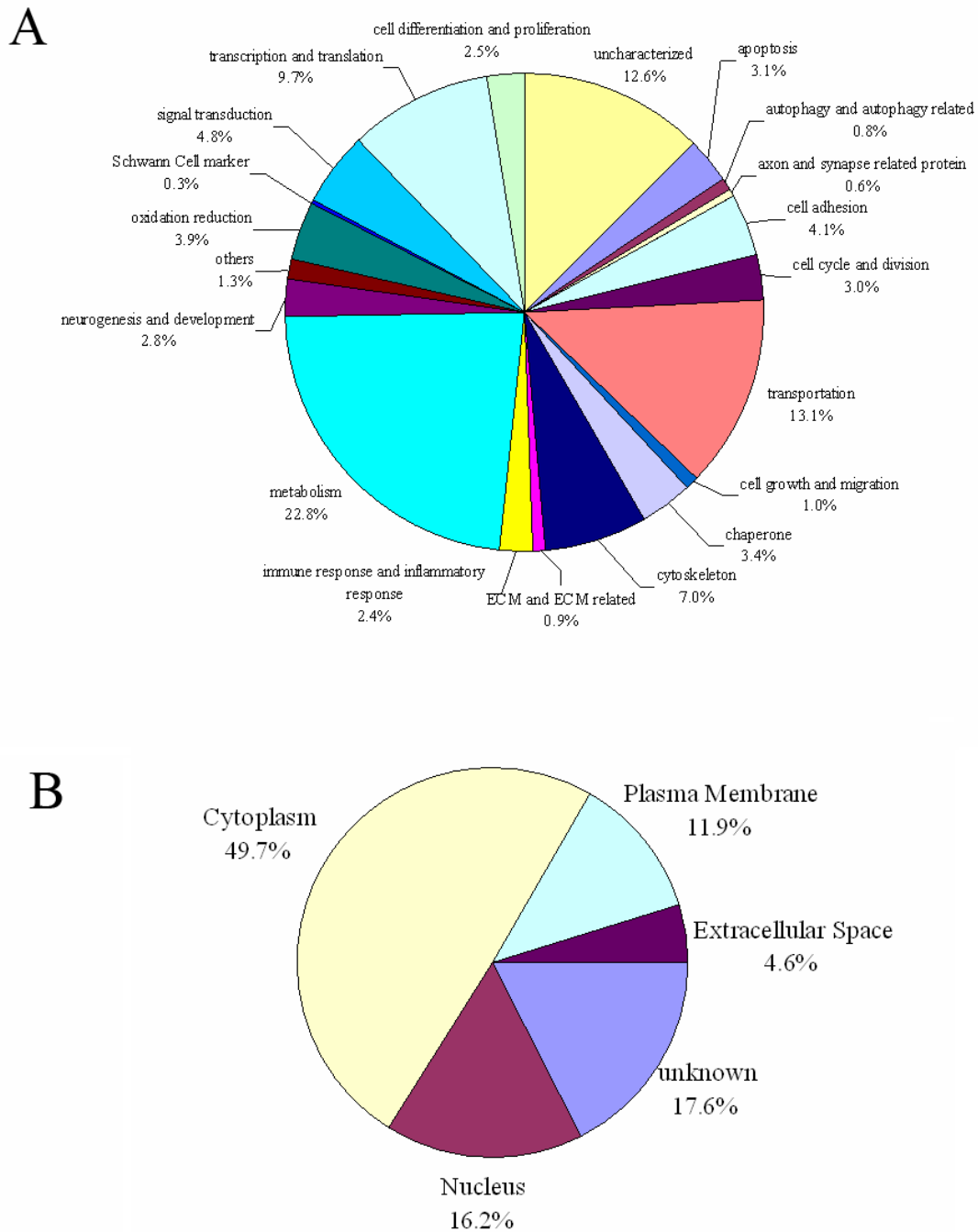
Figure 3 Protein ontology. Identified proteins were classified according to their biological functions (A) and subcellular localization (B).
