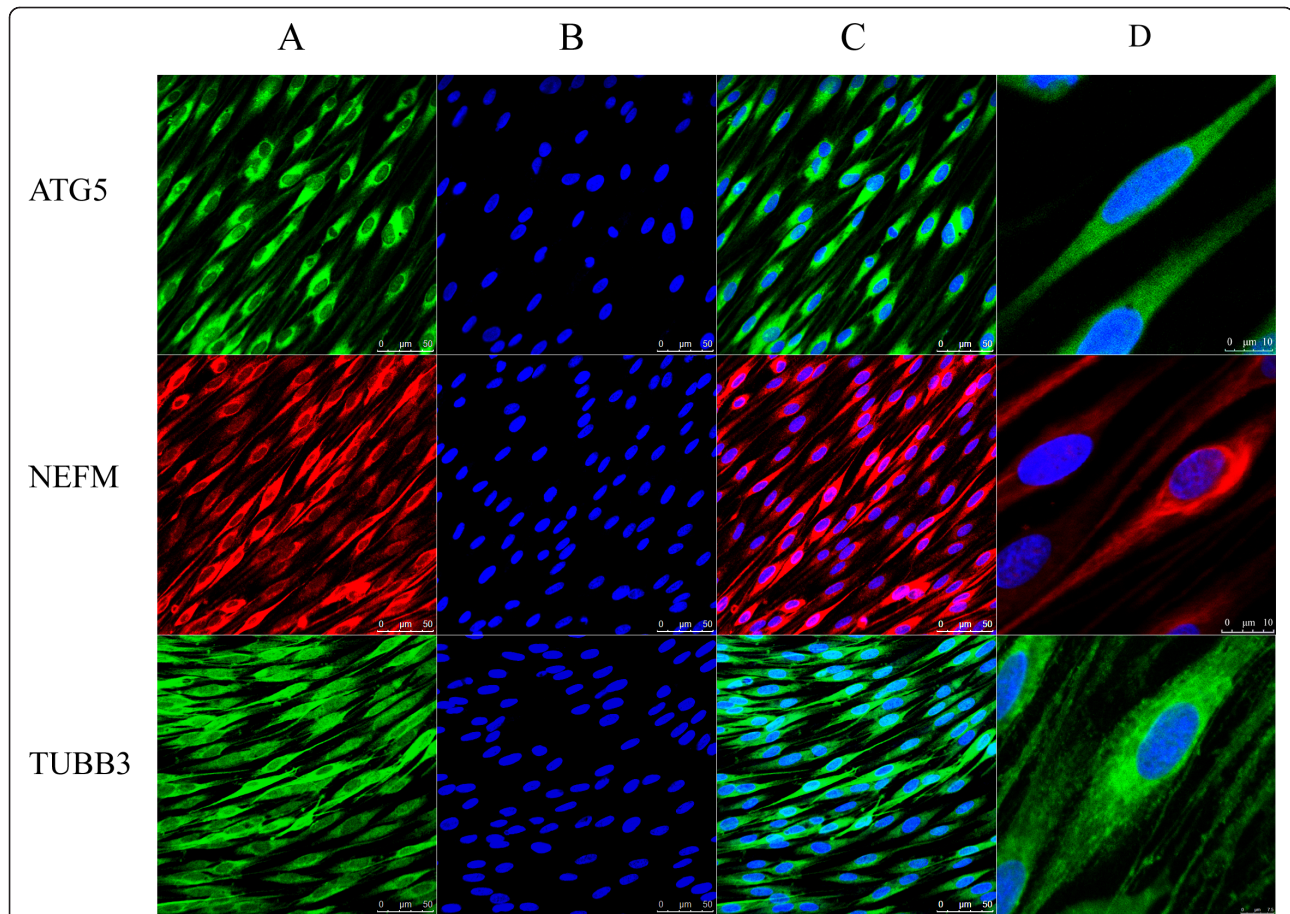
Figure 6 Validation by immunocytochemistry. Light micrographs, taken by a TCS SP5 confocal microscope equipped with a 63 × oil immersion lens, showed that (A) primary culture of SCs were immunostained by antibodies against ATG5 (green color), NEFM (red color), or TUBB3 (green color), respectively; (B) the cell nuclei were stained by Hoechst 33342 (blue color); (C) the merge of (A) and (B); and (D) the views at a much higher magnification of one cell each per antigen. Scale bar as indicated in the images.
