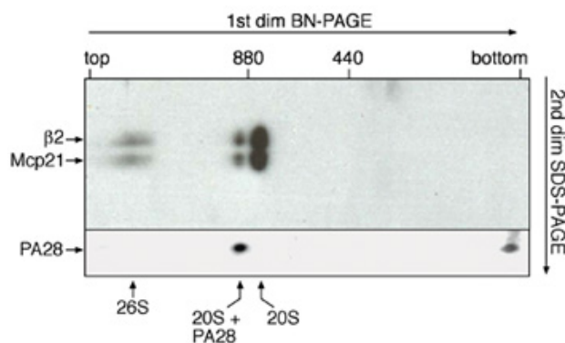
Figure 2. Detection of different forms of the eukaryotic proteasome by immunoblotting after two-dimensional BN-PAGE/SDS-PAGE. For identification and analysis of eukaryotic proteasomes, HEK293 cells were lysed with 0.1% Triton X-100. Cellular lysates were dialyzed and subsequently subjected to BN-PAGE (4-15%) to separate MPCs. Afterwards, a second dimension SDS-PAGE (10%) was run for size separation of individual subcomponents. Immunoblotting was performed with specific antibodies recognizing the Mcp21 and \beta 2 subunit of the 20S core complex, and the regulatory subunit PA28.
