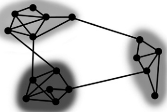
Fig. 1. Graph theory and community detection. Displayed is a depiction of a network, where nodes (solid circles) are connected by edges (solid lines). In this paper nodes are participants and edges are correlations between participants' neuropsychological scores. Community detection algorithms (29) can be applied to graph structures to identify clusters of nodes (shaded clouds) that share many edges within clusters relative to between clusters.
