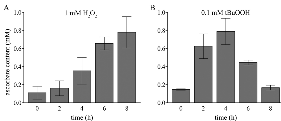
FIGURE 5. Ascorbate levels are elevated in response to oxidative stress. Vitamin C concentration was measured in extracts of C. reinhardtii cells exposed to 1 mM \text{H}_2\text{O}_2 ( A ) or 0.1 mM tBuOOH ( B ) for 2, 4, 6, and 8 h. Error bars represent the S.D. from three biological replicates.
