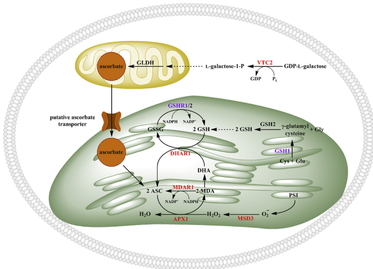
FIGURE 7. Putative regulatory sites for ascorbate biosynthesis and ascorbate recycling in C. reinhardtii . Enzymes depicted in red indicate the proteins whose mRNA levels are increased in response to oxidative stress (1 mM H 2 O 2 and 0.1 mM tBuOOH) and those in magenta that show changes in mRNA levels only in response to H 2 O 2 treatment. APX1 (ascorbate peroxidase), MSD3 (Mn superoxide dismutase), MDAR1 (monodehydroascorbate reductase), DHAR1 (dehydroascorbate reductase), GSH1 ( \gamma -glutamylcysteine synthetase), GSH2 (glutathione synthetase), GSHR1/2 (glutathione reductase), GLDH (L-galactono-1,4-lactone dehydrogenase), VTC2 (GDP-L-galactose phosphorylase), ASC (ascorbate), MDA (monodehydroascorbate), and DHA (dehydroascorbate) are indicated.
