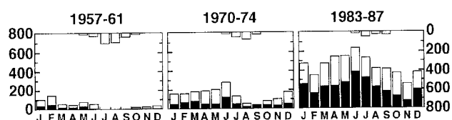
Fig. 10. Mean monthly rainfall and number of hours with visibility reduced to less than 5 km (filled bars) and less than 10 km (empty bars) at Gao during three periods: 1957–1961, 1970–1974, and 1983–1987. The number of hours per month of reduced visibility is on the left-hand vertical axis. The monthly rainfall is shown at the top of each diagram, with the amount in mm indicated on the right-hand vertical axis. [Reproduced with permission from ref. 32 (Copyright 1997, American Meteorological Society)].
