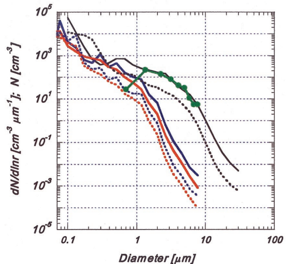
Fig. 8. The particle size distribution during Saharan dust storms. The green points are in situ measurements of dust concentrations made at Tel Aviv during the storm of March 17, 1998. The black lines represent concentrations retrieved from sky radiometers in Sde-Boker (solid line) and Cape Verde (dashed line) during Saharan dust storms. The CCN concentrations are calculated by assuming that all of the vertically integrated particles are concentrated in a 1-km vertical column. The conversion of dust into CCN concentrations is represented by the blue lines (Sde-Boker, solid; Cape Verde, dashed). The red lines (Sde-Boker, solid; Cape Verde, dashed) represent the cumulative concentrations of the CCN, beginning with the largest bin size.
