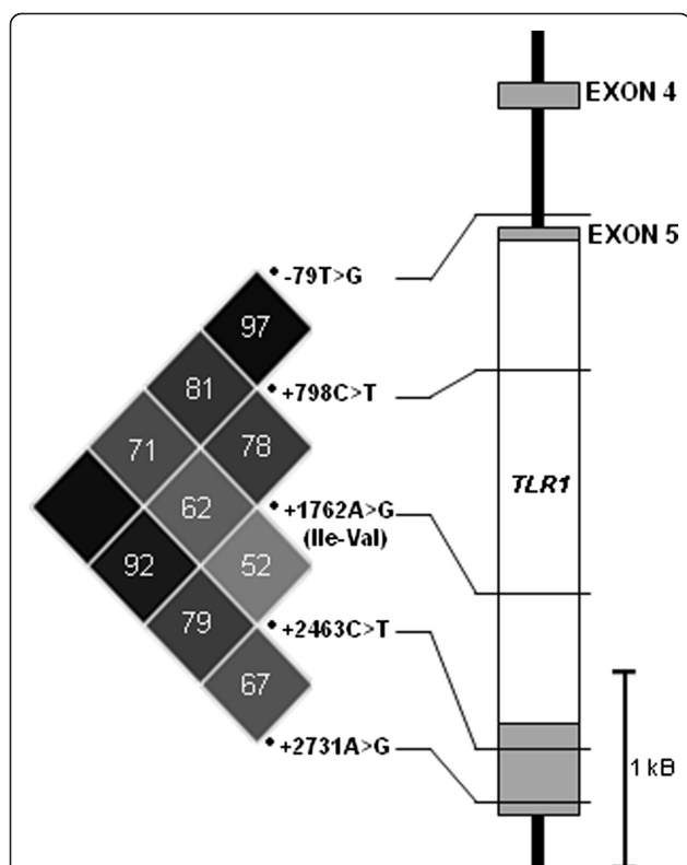
Figure 2 Linkage disequilibrium (LD) plot for five extensively genotyped SNPs in relation to the boTLR1 gene model. Open box represents boTLR1 coding exon, grey boxes represent non-coding untranslated (UTR) exonic regions. The non-synonymous amino acid change is shown in brackets below corresponding coding SNP. The graphical representation, generated by Haploview, of the r^2 LD relationship between each SNP is expressed on a gray-scale gradient; where black - very high LD ( r^2 = 1.0 ) and white - very low LD ( < 0.1 ). The r^2 value for each pair-wise comparison is shown, where no value is indicated r^2 = 1 .
