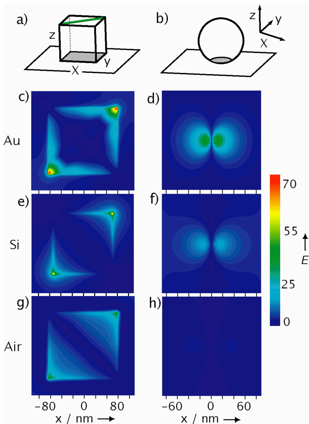
Figure 4. Simulated E-field enhancements for a Ag nanocube or nanosphere. a-b) Schematic of the coordination systems for calculating the E-field enhancement distribution of a nanocube and nanosphere, respectively, positioned 2 nm above a substrate. The grey region represents the plane plotted in the simulations and is 1 nm above the underlying substrate. For nanocube, the polarization was along the green line. The E-field enhancement distributions calculated using the DDA method for: nanocubes c) on Au, e) on Si, and g) in air; as well as for nanospheres d) on Au, f) on Si, and h) in air.
