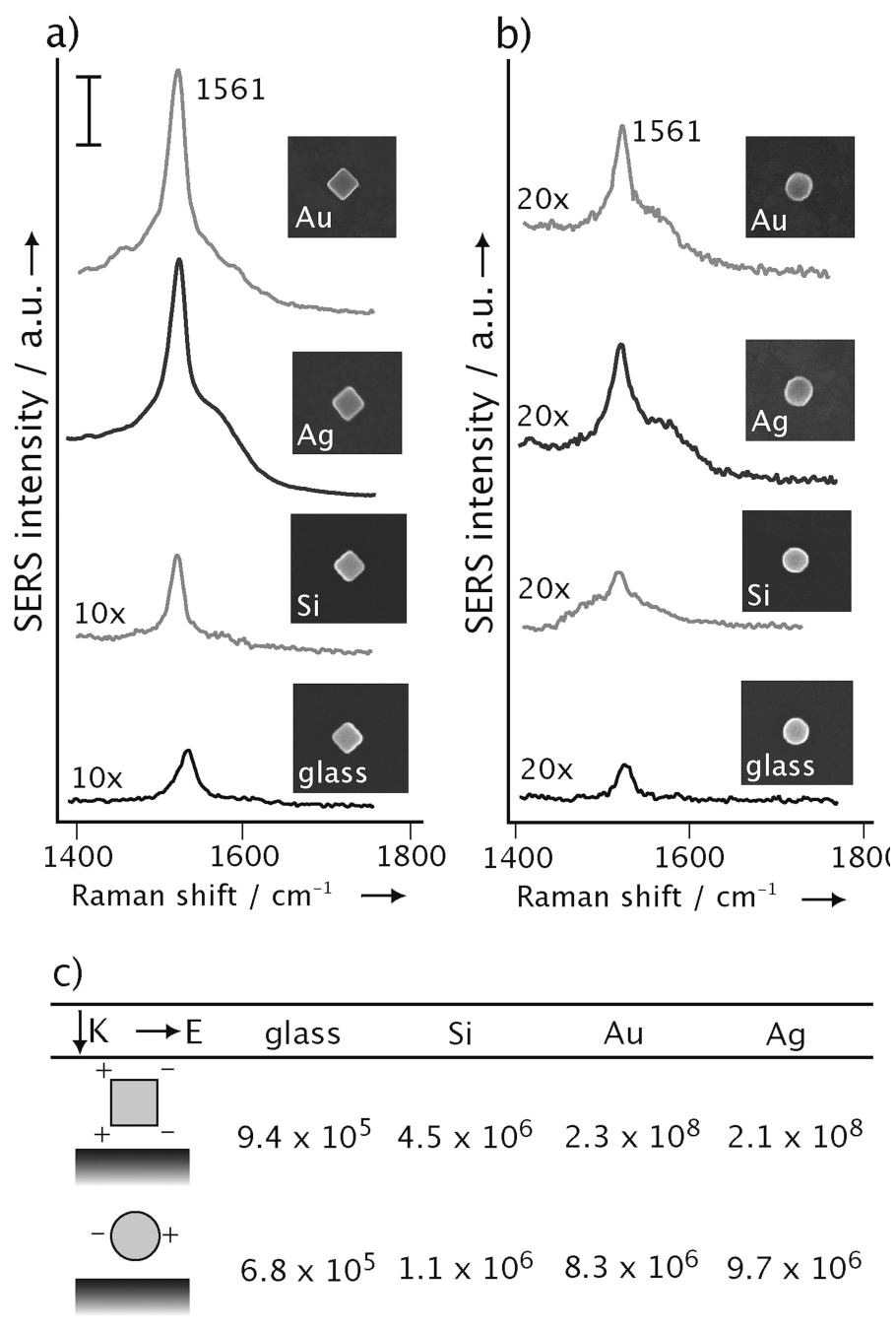
Figure 1. The SERS spectra of 1,4-BDT from: a) nanocubes 106±5 nm in edge length and b) nanospheres 97±7 nm in diameter, on a Au film, Ag film, Si wafer, and glass cover slip, respectively. The insets show their corresponding SEM images. The scale bar for the SERS spectra is 10 adu mW -1 s -1 . c) The EFs for single Ag nanocubes and nanospheres, respectively, supported on different substrates. Each value reported in this table represents an average of the data from 40 particles. The cartoon shows propagation and polarization directions of the laser used in this study and simplified distribution of dipolar charges on each type of particle.
