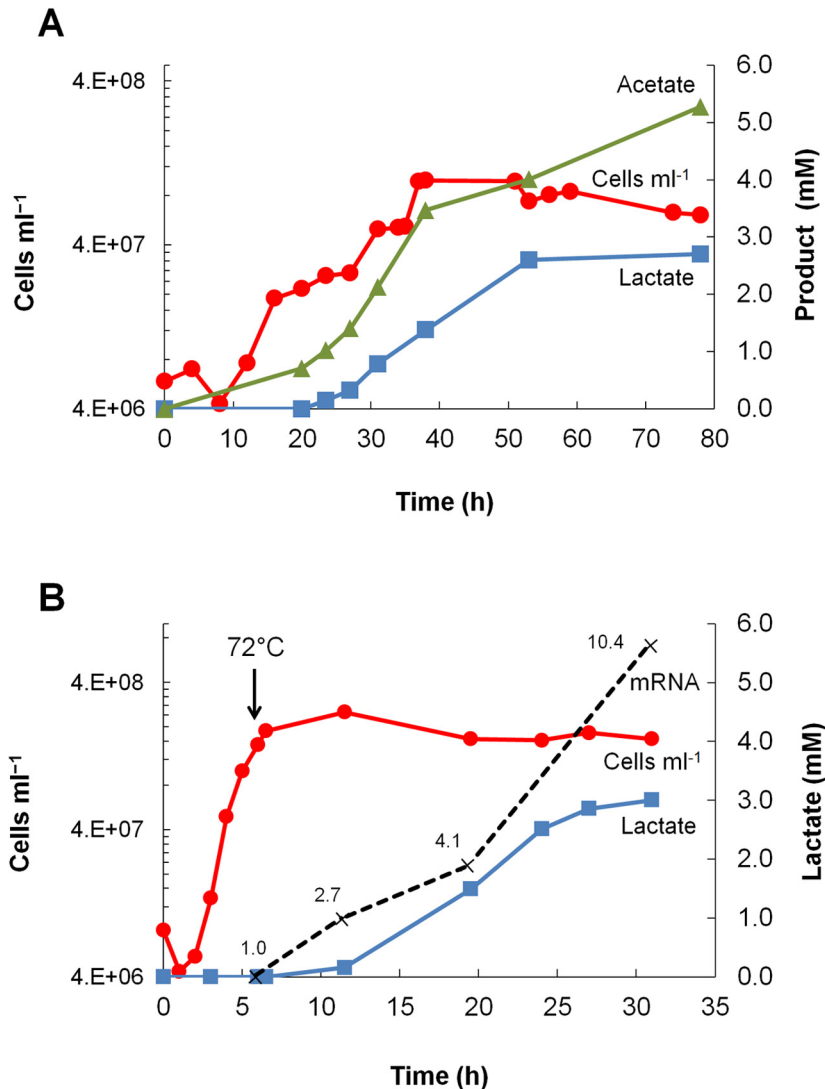
FIG 4 (A and B) Lactate production (blue squares), acetate production (green triangles), cell density (red circles), and relative mRNA fold expression levels (broken lines) in 15-liter fermentor cultures of P. furiosus LAC. One culture was grown at 72°C (A), while another culture was grown at 94°C and rapidly cooled to 72°C after a cell density of 1.5 \times 10^8 was reached (indicated by the black arrow) (B). After the temperature switch, higher mRNA levels for the heterologous gene Cbes-ldh , high specific activity of lactate dehydrogenase, and a high rate of lactate formation were observed.
