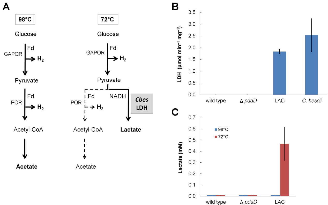
FIG 1 Recombinant expression of lactate dehydrogenase (LDH) in P. furiosus strain LAC changes its fermentation pattern. (A) Concept of temperature-dependent switch in end product formation by P. furiosus . Abbreviations: GAPOR, glyceraldehyde-3-phosphate ferredoxin oxidoreductase; POR, pyruvate ferredoxin oxidoreductase; Fd, ferredoxin; acetyl-CoA, acetyl coenzyme A; Cbes LDH, C. bescii LDH. (B) Specific activity of lactate dehydrogenase in the protein extract of C. bescii DSM 6725, P. furiosus DSM 3638 (wild type), P. furiosus \Delta pdaD host strain, and P. furiosus LAC obtained from 400-ml batch cultures. (C) Lactate production in the same P. furiosus cultures. Values given are averages \pm standard deviations (SD) (error bars) of three independent biological cultures.
