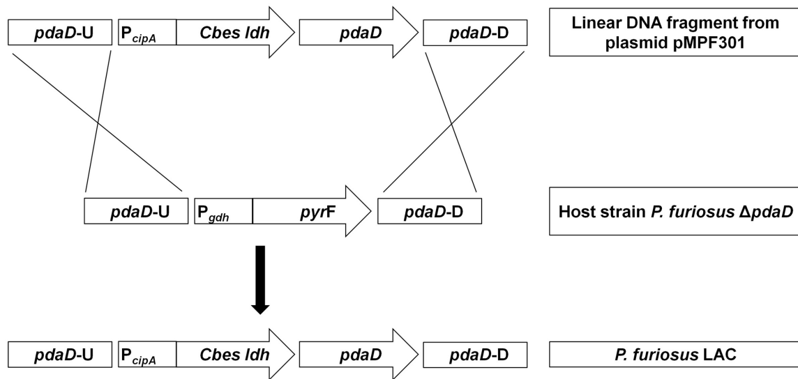
FIG 3 Cloning strategy for the mutant strain P. furiosus LAC. The fusion product P cipA Cbes-ldh was obtained by overlapping PCR and integrated into vector pSPF300 (11). The new vector, pMPF301 (Fig. 2), additionally carried the pdaD gene essential for agmatine biosynthesis and 1-kb upstream and downstream flanking regions of the pdaD gene. Linearized DNA was used for transformation of the P. furiosus Δ pdaD host strain. The pdaD P cipA Cbes-ldh cassette integrated into the genome by homologous recombination, replacing the P gdh pyrF cassette. Therefore, the resulting new strain, P. furiosus LAC, exhibits a uracil auxotrophy, but does not, in contrast to the host, require agmatine for growth.
