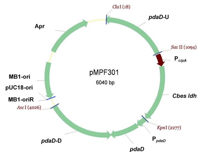
FIG 2 Plasmid vector pMPF301 containing the pdaD P cipA Cbes-ldh cassette, 1-kb upstream and downstream flanking regions of the pdaD gene and the apr gene as a selective marker in Escherichia coli (apramycin resistance). Plasmid diagrams were constructed using Vector NTI software (Invitrogen).
