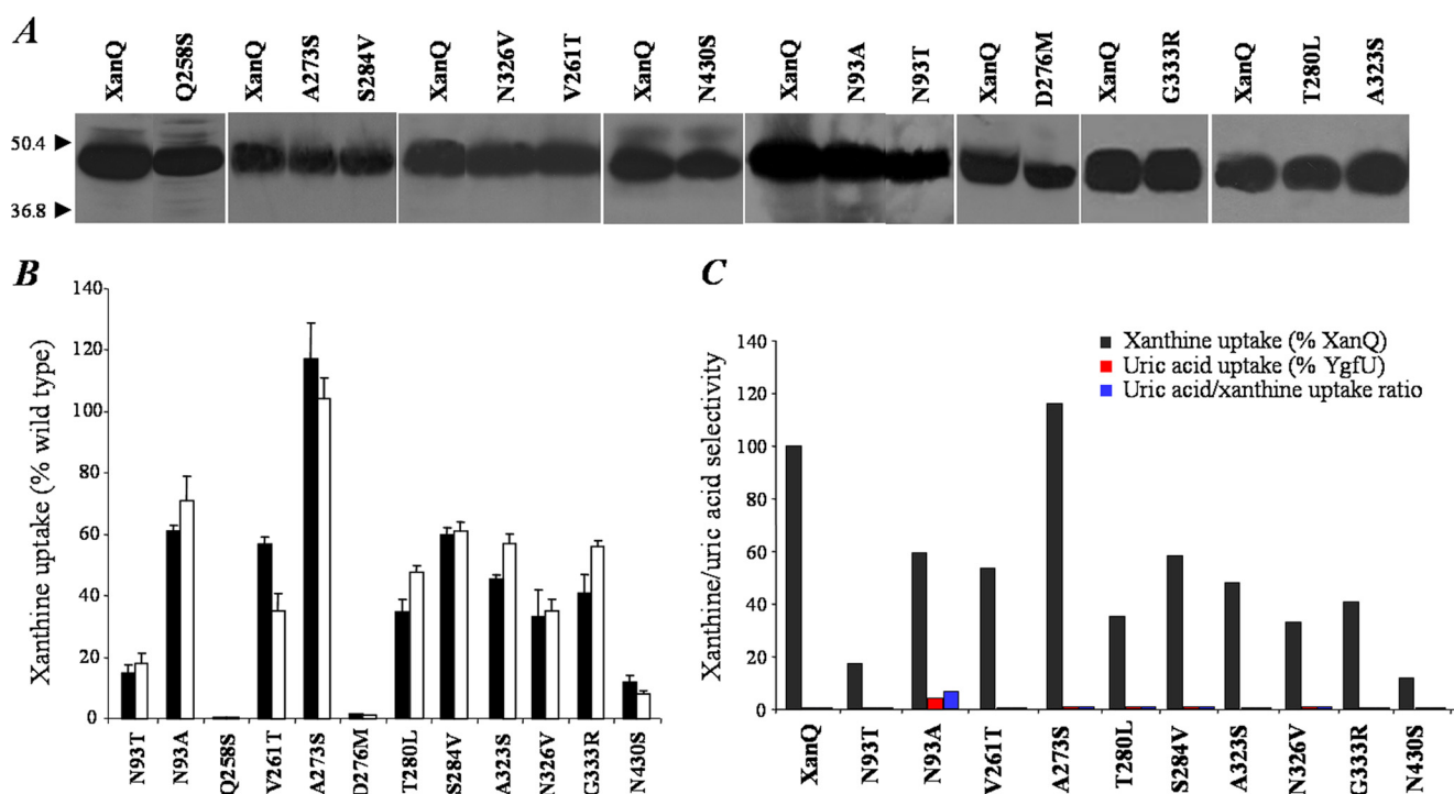
FIGURE 6. Expression and uptake activities of XanQ mutants. E. coli T184 harboring pT7-5/ xanQ (wild-type-BAD) with given mutations were grown, induced, and subjected to immunoblot analysis of membrane fractions (A) or assayed for transport of [ 3 H]xanthine (1 \mu M, 25 °C) (B) and [ 14 C]uric acid (2 mM, 25 °C) (C), exactly as described in the legend for Fig. 4. Closed and open histogram bars represent initial rate and steady-state values, respectively. Results are expressed as a percentage of the activity of wild-type control with standard deviations from three independent determinations.
