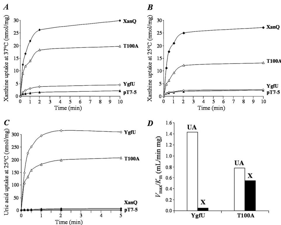
FIGURE 5. Analysis of substrate selectivity for mutant T100A. E. coli T184 harboring pT7-5/ ygfU (wild-type-BAD), pT7-5/ ygfU (T100A-BAD), pT7-5/ xanQ (wild-type-BAD), or pT7-5 alone were grown, induced, and assayed for transport of [ 14 C]uric acid (0.01–2 mM, 25 °C) and [ 3 H]xanthine (0.1 μM–0.25 mM, 37 °C or 25 °C), as described in the legends for Fig. 4 and Table 1. A, time courses of xanthine (0.1 mM) uptake at 37 °C. B, time courses of xanthine (0.1 mM) uptake at 25 °C. C, time courses of uric acid (1 mM) uptake at 25 °C. D, comparison of the transport efficiencies ( V_{max}/K_m ) for uric acid (25 °C) and xanthine (37 °C) displayed by YgfU and T100A (see also Table 1). The abbreviations are: UA, uric acid; and X, xanthine.
