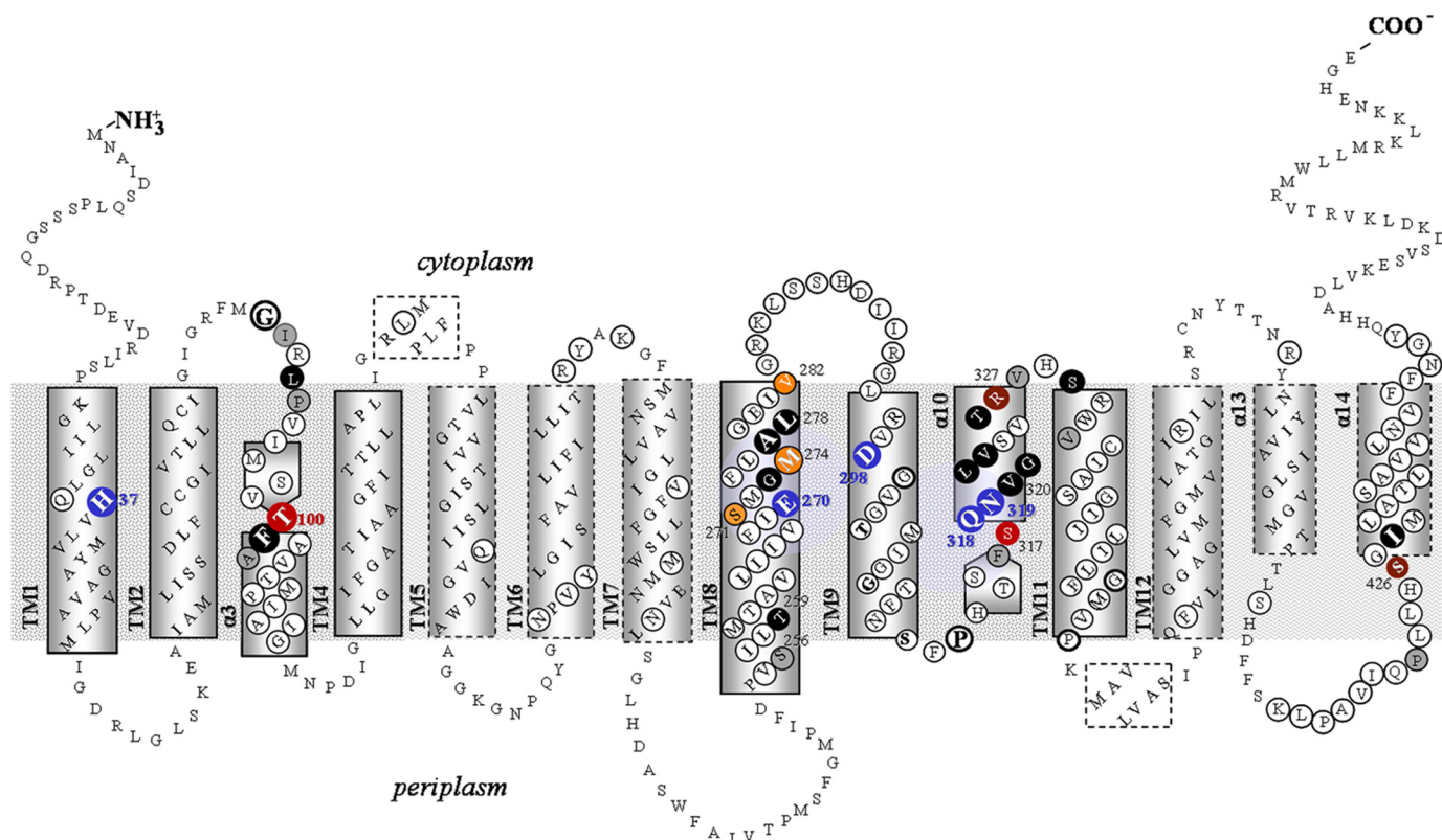
FIGURE 3. Topology model of YgfU permease and mutagenesis targets. The model is derived from homology threading using the UraA structure (3QE7) as a template and initial topology predictions based on the program TMHMM and analysis of the XanQ homolog for the accessibility of loops to hydrophilic reagents (8). The \alpha -helical segments are indicated in rectangles with continuous line (core domain) or broken line perimeters (gate domain). Residues corresponding to the ones analyzed with Cys-scanning mutagenesis in XanQ are circled . Residues corresponding to the important set (Fig. 2) are shown in a dark background (functionally important in XanQ) or in a bold circle (crucial for expression in XanQ). Residues corresponding to positions of XanQ mutants that are moderately sensitive to N -ethylmaleimide ( IC_{50} values from 100 \mu M to 1 mM) are in a gray background . The residues of YgfU analyzed in this study with site-directed mutagenesis are numbered and shown in blue (irreplaceable for function), red (essential for the counter-selectivity against xanthine), dark red (replacements lead to lower affinity for uric acid), orange (replacements lead to abolishment of expression in the membrane), or gray scale (remaining positions).
