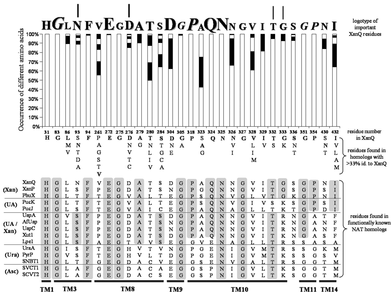
FIGURE 2. Conservation pattern of important residues of XanQ in NAT family. A logotype of 29 residues delineated as important from the Cys-scanning analysis of XanQ (5–10) is shown on top. Larger sized letters indicate irreplaceable XanQ residues, medium sized letters indicate residues that are replaceable with a limited number of side chains, and smaller sized letters indicate residues where a Cys replacement is highly sensitive to inactivation by N -ethylmaleimide ( IC_{50} < 100 \mu\text{M} ). A perpendicular line indicates a residue where replacements distort specificity for the imidazole moiety of substrate (leading to aberrant recognition of uric acid and 8-methylxanthine). Italics indicate residues that are crucial (smaller size) or irreplaceable (larger size) for expression in the membrane. The histogram in the upper panel shows the number and relative abundance of different amino acids found at each position of the important set in the 189 closest homologs (>33% sequence identity with XanQ) (10); the corresponding variants are listed in decreasing order of frequency, whereas variants with very low occurrence ( \leq 1.6\% ) are omitted for clarity. The sequence alignments in the lower panel show the residues found at each position of the important set in 15 characterized NAT/NCS2 transporters, including E. coli XanQ (P67444), XanP (POAGM9) and UraA (POAGM7), B. subtilis PbuX (P42086), PucK (O32140) and PucJ (O32139), Lactococcus lactis PyrP (AAK05701), A. nidulans UapA (Q07307) and UapC (P487777), Aspergillus fumigatus AfUapA (XP748919), Candida albicans Xut1 (AAX2221), Zea mays Lpe1 (AAB17501), Homo sapiens SVCT1 (SLC23A1) (AAH50261) and SVCT2 (SLC23A2) (Q9UGH3), and Rattus norvegicus SNBT1 (SLC23A4) (AB511909). The full-length sequences were aligned using ClustalW, and part of this alignment including the residues of interest is presented. Major substrates of each transporter are shown in parentheses on the left. The abbreviations are: Xan , xanthine; UA , uric acid; Ura , uracil; and Asc , ascorbate.
