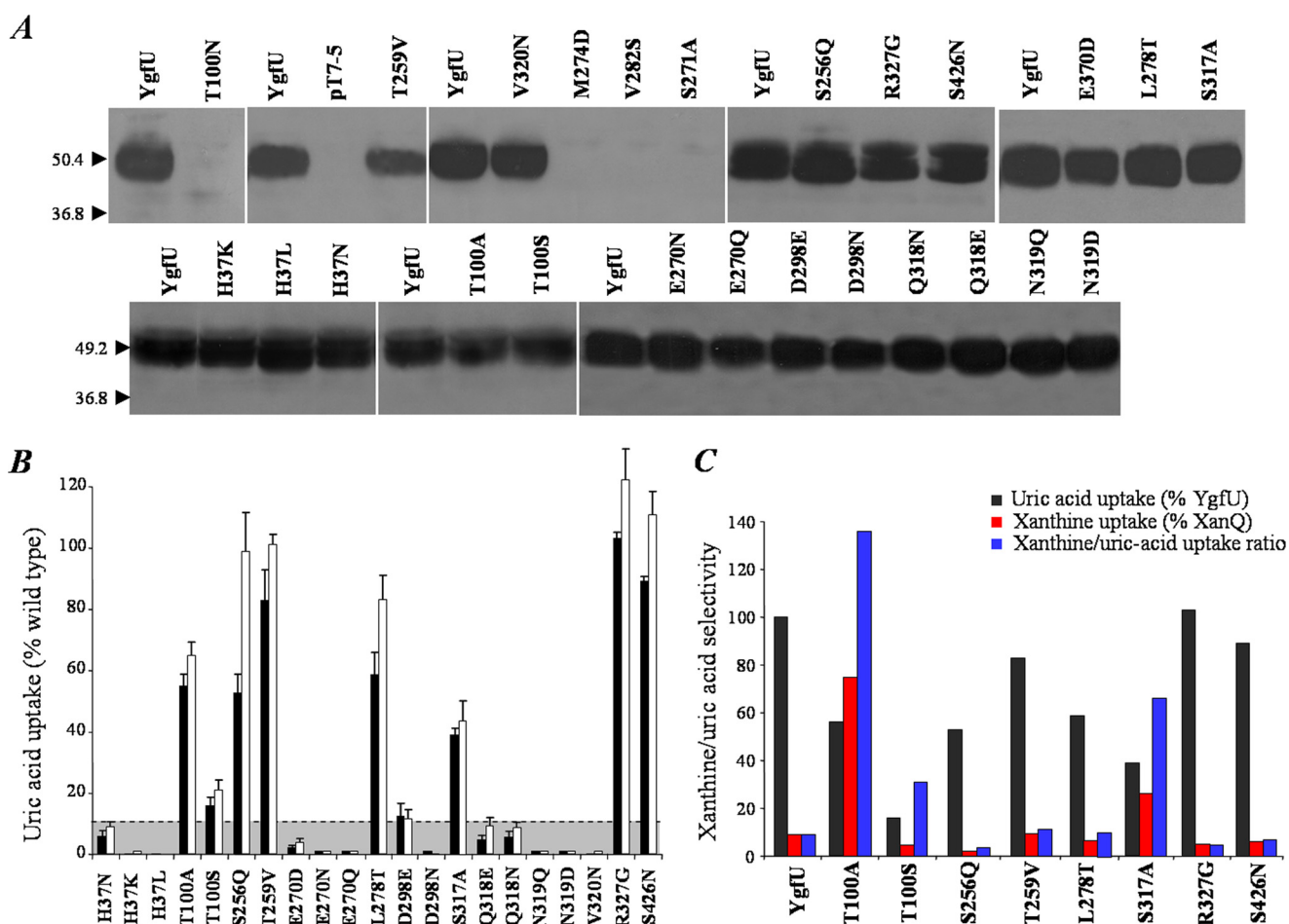
FIGURE 4. Expression and uptake activities of YgfU mutants. E. coli T184 harboring pT7-5/ygfU(wild-type-BAD) with given mutations were grown aerobically to mid-logarithmic phase, induced with isopropyl-1-thio- \beta -D-galactopyranoside (0.5 mM) for 2 h, and subjected to immunoblot analysis of membrane fractions to mid-logarithmic phase, induced with isopropyl-1-thio- \beta -D-galactopyranoside (0.5 mM) for 2 h, and subjected to immunoblot analysis of membrane fractions or assayed for transport of [ ^{14} C]uric acid (1 mM, 25 °C) and [ ^3 H]xanthine (0.1 mM, 37 °C). A , samples containing ~100 \mu g of membrane protein were subjected to SDS-PAGE (12%) and immunoblotting using HRP-conjugated avidin. Prestained molecular mass standards (in kDa; Bio-Rad, low range) are shown on the left. B , initial rates of uric acid uptake (closed histogram bars) were measured at 5–15 s, and steady-state levels of uric acid accumulation (open histogram bars) were measured at 2–10 min. Control values obtained from T184 harboring pT7-5 alone were subtracted from the sample measurements in all cases. Results are expressed as a percentage of the activity of wild-type control with standard deviations from three independent determinations. C , comparison of initial rates of uric acid and xanthine uptake for the active YgfU mutants. Results are expressed as a percentage of the rate of YgfU and XanQ, respectively. The percentage ratio of the xanthine uptake value (red) to the uric acid uptake value (black) is given for each mutant in a third histogram bar (blue).
