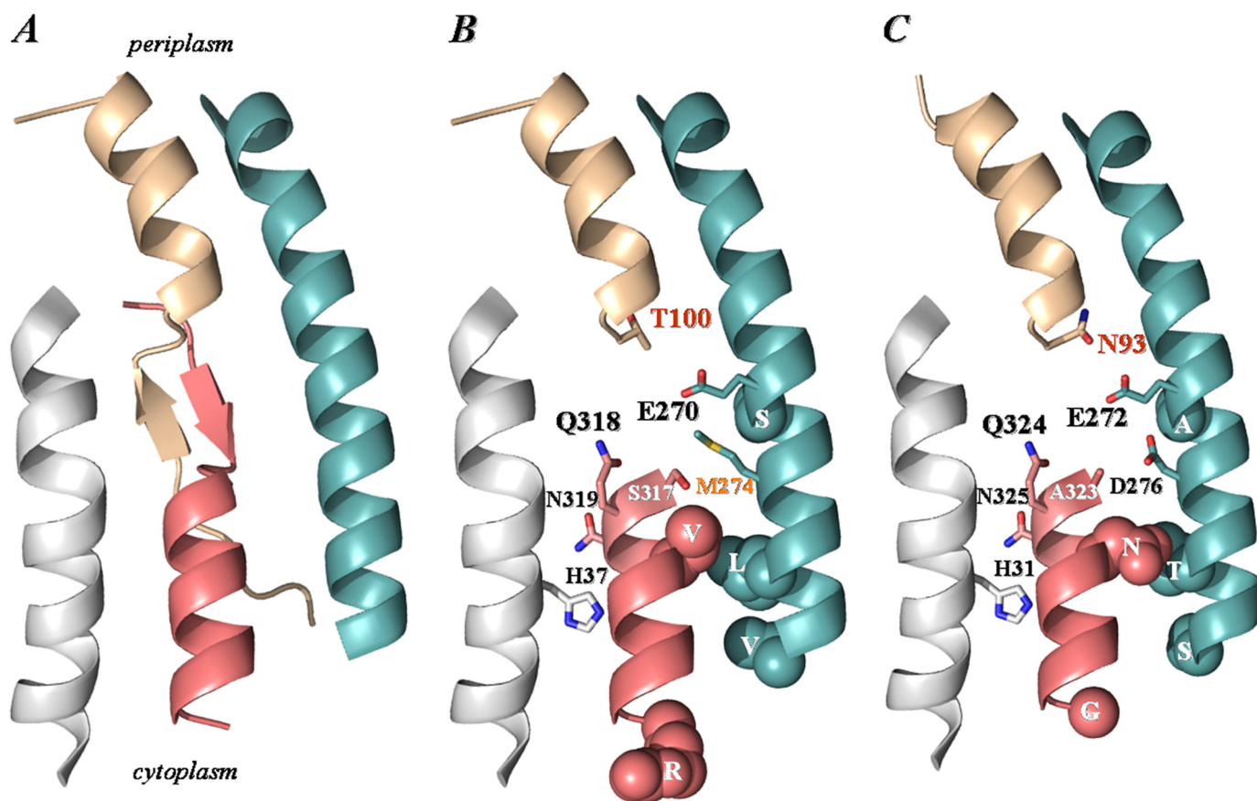
FIGURE 7. Arrangement of important residues in modeled structure of YgfU. The sequences of YgfU and XanQ were threaded on the known x-ray structure of UraA (1) using the SWISSPROT modeling server. The structural models were displayed with PyMOL version 1.4. Shown are four TMs that contain binding residues and form a shelter around substrate in UraA, namely TM1 (gray), TM3 (wheat), TM8 (teal), and TM10 (salmon). A, arrangement of the four TMs in the YgfU model. B, the same model (YgfU) excluding the \beta -strand regions of TM3 and TM10 and indicating the side chains of residues analyzed with mutagenesis in this study. C, arrangement of the corresponding residues and helices in XanQ. The side chains of important residues of YgfU (B) and XanQ (C) are shown as thick sticks (irreplaceable and/or substrate binding-relevant) or spheres (sensitive to alkylation or bulky replacement in XanQ; crucial for the protein expression or affinity in YgfU). The side chain of Thr-100 (or Asn-93), which is associated with the uric acid selectivity, is shown with red label.
