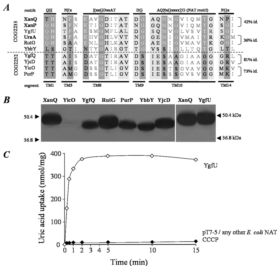
FIGURE 1. Sequence, immunoblot, and nucleobase uptake analysis of NAT homologs from E. coli K-12 were aligned using ClustalW, and part of this alignment referring to conserved sequence motifs of the family is shown in A . The members include the known nucleobase transporters XanQ (P67444), XanP (P0AGM9), and UraA (P0AGM7) and the unknown YgfU (Q46821), RutG (P75892), YbbY (P77328), YgfQ (Q46817), YjcD (P0AF52), YicO (P31440), and PurP (P31466). The motifs shown are characteristic for functionally known members of the family and have been shown to contain functionally important residues in XanQ (6–10). Sequence identity scores are shown on the right . The coding sequences from the unknown homologs were mobilized from the genome, induced for overexpression in E. coli T184 under control of the lacZ promoter/operator in pT7-5/NAT-BAD, and assayed for expression levels in the membrane and active transport of xanthine, uracil, and uric acid. B , samples containing 100 \mu g of membrane protein were subjected to SDS-PAGE (12%) and immunoblotting using HRP-conjugated avidin. C , cells expressing each homolog were normalized to 0.7 mg of protein/ml of cell suspension and assayed for active transport of [ ^{14} C]uric acid (1 mM, 25 ^{\circ} C) in the presence or absence of carbonyl cyanide m -chlorophenyl hydrazone (CCCP) (10 \mu M). Transport assays were also performed for [ ^3 H]xanthine (1 \mu M, 25 ^{\circ} C), using XanQ as a positive control (4), and for [ ^3 H]uracil (1 \mu M, 25 ^{\circ} C). Uracil uptake could not be detected with any of the unknown homologs; xanthine uptake was observed only with RutG, albeit to a marginal extent (not shown).
