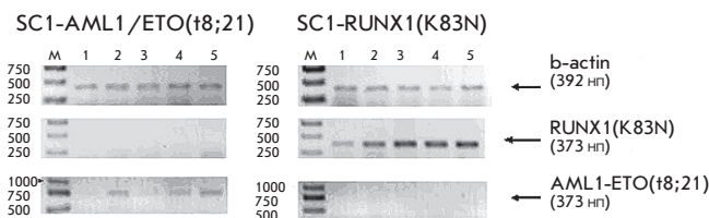
Fig. 3. The electrophoregram of RT-PCR products of total cDNA obtained from oncogene expressing model cell lines transfected with siRNA. 1) siRNA(AML1-5'), 2. siRNA(AML1-3'), 3. siRNA(AML1-ETO), 4. siRNA(ETO), 5. Control (without siRNA)
