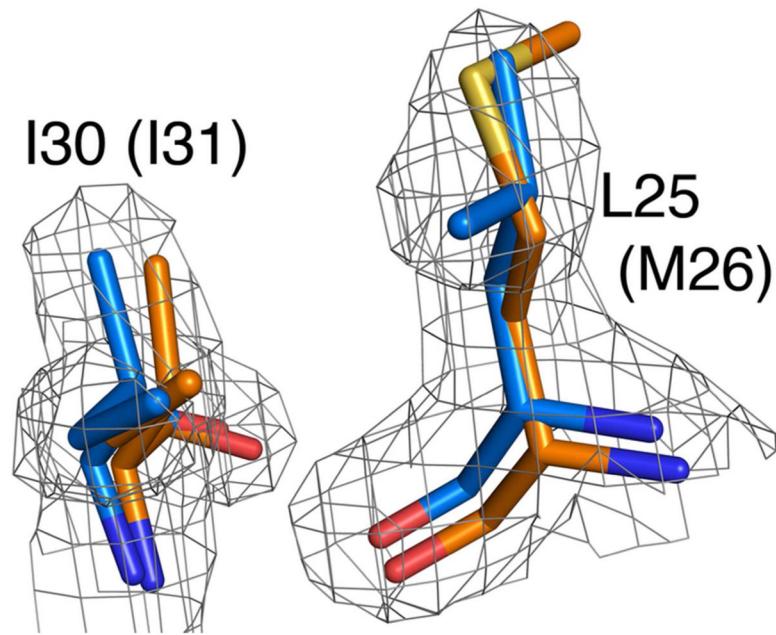
Figure 2. The parkinsonism-associated Met26 residue is replaced with a structurally conservative leucine residue in DJ-1β. A stick representation of the superimposed structures of human DJ-1 (orange) and Drosophila DJ-1β (blue) shows that the substitution of leucine for methionine causes minimal structural disruption in that area, in contrast to packing defects created by the M26I mutation in human DJ-1. Drosophila DJ-1β numbering is shown with human residue numbering in parenthesis.
