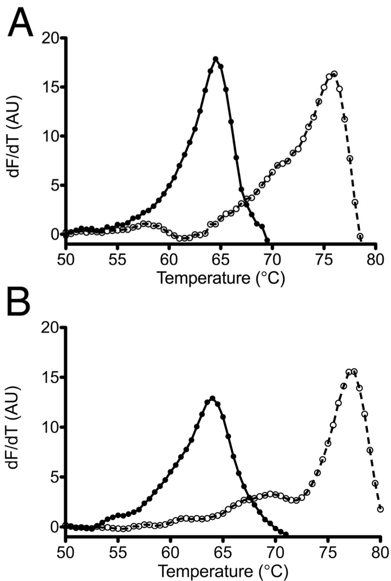
Figure 5. Cysteine-sulfinate formation stabilizes DJ-1. The thermofluor assay was used to monitor the thermal denaturation of reduced DJ-1 (filled circles) or protein that was oxidized at the conserved cysteine residue to the cysteine-sulfinate (open circles). Drosophila DJ-1 \beta is shown in panel A and human DJ-1 is in panel B. In both cases, oxidation increases the thermal stabilities of the proteins by \sim 12^{\circ}\text{C} .
