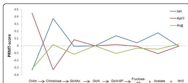
Figure 5 PRMT-scores for chitin catabolism subnetwork. PRMT-scores for metabolites along the chitin catabolism subnetwork are grouped by time point of metagenomic sample. Positive PRMT-scores indicate a predicted increase in relative catabolism, and negative PRMT-scores indicate a predicted increase in synthesis of a metabolite.
