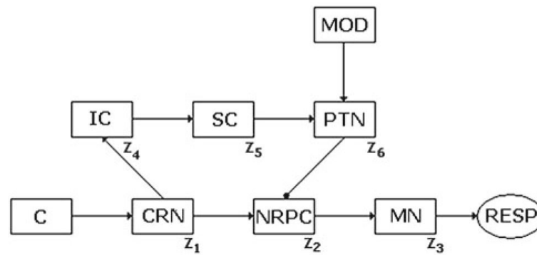
Fig. 1. Network for ASR and PPI: C cochlea, CRN cochlear root nucleus, NRPC nucleus reticularis pontine caudalis, IC inferior colliculus, SC superior colliculus, PTN pontine tegmental nucleus, MN motor neurons, RESP motor response, MOD modulatory network
