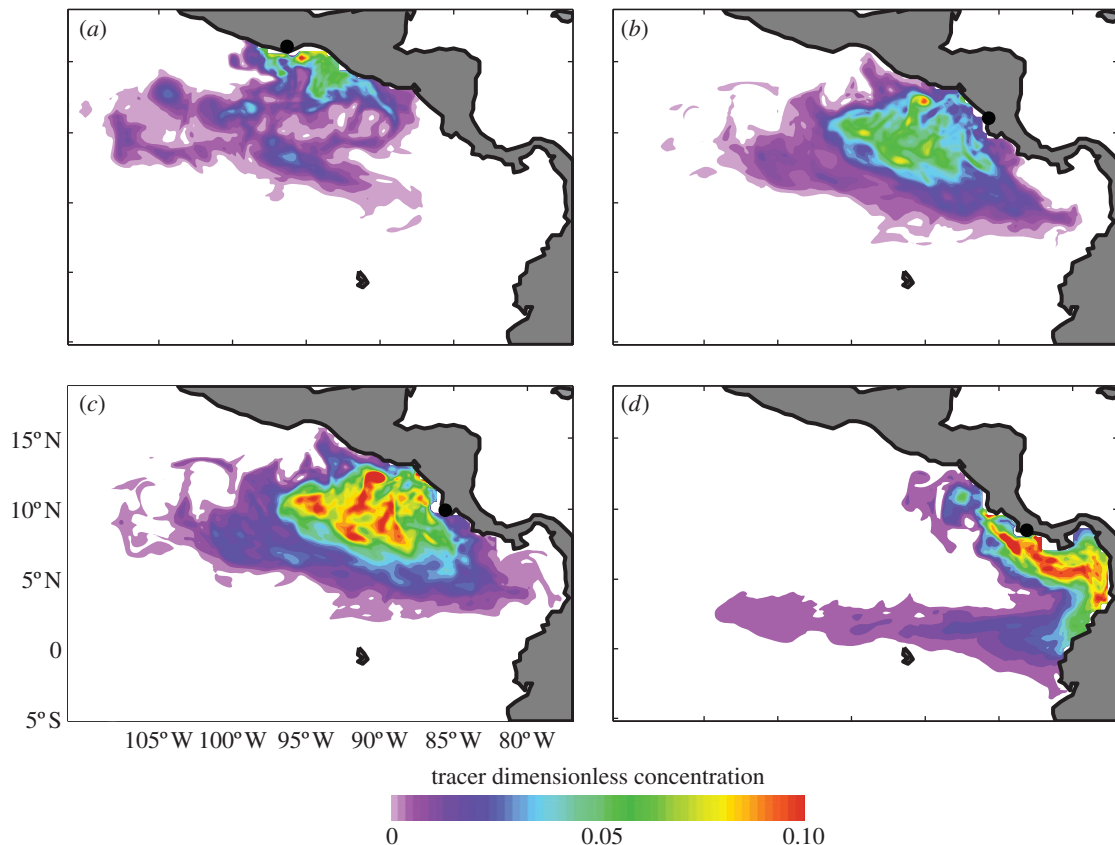
Figure 2. Long-term (2000–2008) mean tracer concentration at 1 June based on continuous tracer releases between 15 January and 15 April from nesting beaches at (a) Barra de la Cruz, (b) Playa Chacocente, (c) Playa Grande and (d) Playa Carate. Black dots show tracer release locations.
