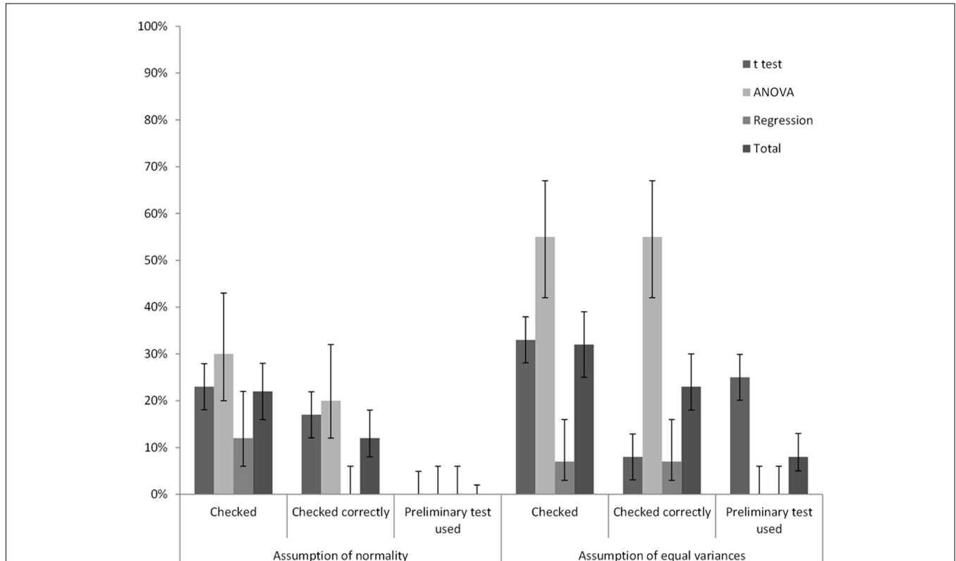
FIGURE 2 | The frequency of whether two assumptions were checked at all, whether they were checked correctly, and whether a preliminary test was used for three often used techniques in percentages of the total number of cases. Between brackets are 95% CIs for the percentages.
