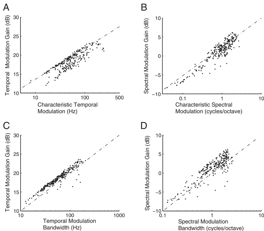
Figure 6. Modulation gains increase systematically with characteristic modulation frequencies and bandwidths. A , Temporal modulation gain is strongly correlated with cTMF ( r = 0.79 \pm 0.02 , p < 0.01 ) while spectral modulation gains are strongly correlated with cSMF ( r = 0.78 \pm 0.03 , p < 0.01 ). These trends are even stronger when one considers the relationship between modulation gains and modulation bandwidths. C , D , As can be seen there is a marked correlation between these parameters ( C , r = 0.95 \pm 0.01 , p < 0.01 ; D , r = 0.94 \pm 0.02 , p < 0.01 ) and a significant increase in power with modulation frequency (7.65 dB/decade for temporal; 8.2 dB/decade for spectral). These trends oppose the MPS of natural sounds where the modulation power decreases with modulation frequency (Fig. 2C,D).
