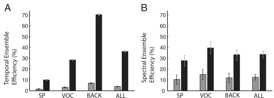
Figure 8. CNIC filtering characteristics enhance encoding efficiency for natural sound ensembles. A , Temporal ensemble efficiency for an equal resolution filterbank (gray) and a proportional resolution filterbank where filter bandwidths scale as for CNIC (black). The CNIC filterbank exhibits significantly higher temporal efficiency ( p < 0.01 , bootstrap t test) for all three natural sound ensembles tested (SP, speech; VOC, animal vocalizations; BACK, background; ALL, SP + VOC + BACK). B , Spectral encoding efficiency is shown for the equal resolution filterbank (gray) and CNIC model filterbank (black). The spectral ensemble efficiency is significantly higher for the CNIC model filterbank for all natural sound ensembles tested ( p < 0.01 , bootstrap t test). Error bars designate SEM.
