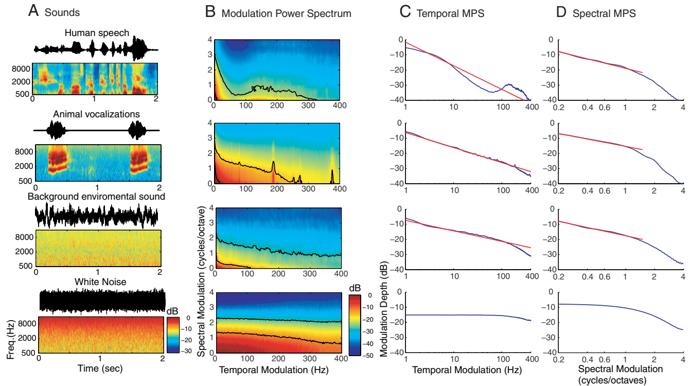
Figure 2. Ensemble characteristics of natural sounds. Natural sounds waveforms ( A , black waveforms) were decomposed by an auditory filterbank model into a spectrotemporal representation ( A , color panels) that depicts the sound power as a function of time and frequency. Representative 2 s segments from speech (male speaker; “If she unmask her beauty to the moon.”), an animal vocalization (wild cat; Felis herpailurus yaguarondi ), background sound (rain), and white noise (top to bottom). For vocalizations the sound power is coherently modulated over frequency and time, whereas for background sounds and white noise the modulations are random. For white noise the power at high frequencies is accentuated because the auditory filterbank bandwidths are larger for higher frequencies. B , The MPS depicts the signal power as a function of temporal and spectral modulation frequency. Black contours in the MPS denote the modulation space that accounts for 90% and 50% of the MPS power. For all three natural sounds, a tradeoff between temporal and spectral modulations is observed. C, D , The temporal and spectral modulation power spectrum was obtained by decomposing the MPS into its strictly spectral and temporal components (see Materials and Methods). A strong decrease in the modulation power of all natural sounds approximates a power law (straight line on a doubly logarithmic plot). A comparable decrease in the modulation power is not observed for white noise. Red curves in C and D designate the optimal-fit power law.
