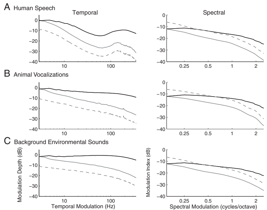
Figure 7. CNIC filtering characteristics equalize the modulation power of natural sounds. A–C show the temporal (left) and spectral (right) MPS (dashed gray lines) for the three natural sound ensembles (human speech, animal vocalizations and background environmental sounds; same as in Fig. 2). To determine the degree of power equalization conferred by the CNIC ensemble, the MPS of natural sounds were passed through a modulation filterbank in which modulation bandwidths scale as for the CNIC neural ensemble (see Materials and Methods). Black lines in A–C represent the CNIC model filterbank output MPS. For reference the MPS were also filtered with an equal resolution filterbank analogous to Figure 1A (gray lines). There is marked flattening in the modulation power at the output of the CNIC model but not for the equal resolution filters.
