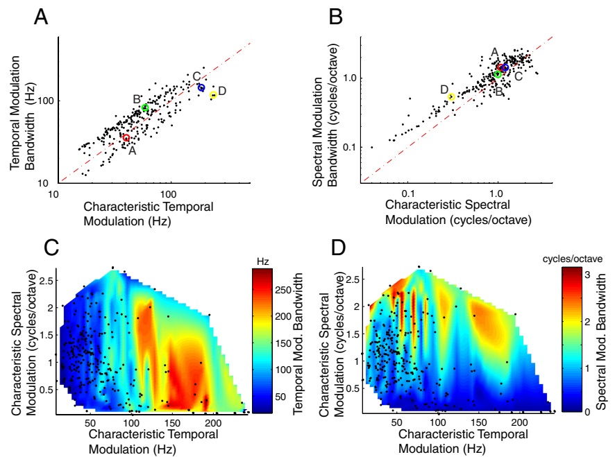
Figure 5. Modulation tuning characteristics in the CNIC. A, B , Temporal and spectral modulation bandwidths show a clear increase as function of their respective characteristic modulation frequency (slope of increment for temporal: 0.8, p < 0.01 ; spectral: 0.75, p < 0.01 ). The selected examples from Figure 3 are indicated by A–D . C and D show the relationship between temporal ( C ) and spectral ( D ) modulation bandwidths (surface color plots) as function of cTMF and cSMF (black dots, indicate the cTMF and cSMF of each neuron). Note that temporal modulation bandwidths scale most prominently with cTMF. Likewise, spectral modulation bandwidths scale most prominently with cSMF.
