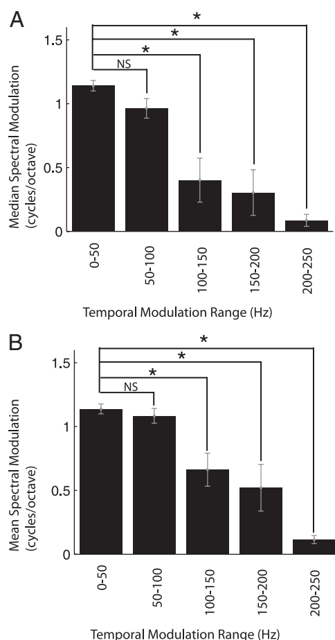
Figure 4. Modulation tradeoff statistics. A, B , Median ( A ) and mean ( B ) cSMF as a function of cTMF range. The neural ensemble was partitioned into nonoverlapping cTMF ranges (0–50, 50–100, 100–150, 150–200, 200–250 Hz). Both the median and mean cSMF decreased systematically with increasing cTMF range. Error bars designate the bootstrapped SE and * designates significant results (median, Wilcoxon rank-sum, p < 0.05 with Bonferroni correction; mean, paired t test, p < 0.05 with Bonferroni correction).
