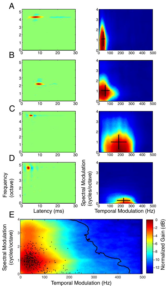
Figure 3. Tradeoff in neural spectrotemporal tuning in the inferior colliculus. A–D , Example STRF and the corresponding MTFs from four CNIC neurons. The example STRFs ( A–D , left) are ordered from slow to fast integration times ( A , 6.6 ms; B , 3.92 ms; C , 2.12 ms; D , 2.13 ms). The STRF bandwidths for these examples represent the average width of the STRF ( A , 0.20 octave; B , 0.25 octave; C , 0.18 octave; D , 0.43 octave). As can be seen, neurons can be sharply or broadly tuned in frequency or can alternately exhibit short or long integration times. The STRF structure is directly related to the modulation tuning characteristics of each neuron ( A–D , MTF shown on right). STRFs with slow integration times ( A ) prefer slower temporal modulation while faster STRFs prefer higher temporal modulations ( D ). Similarly, narrowband STRFs with strong side-band inhibition tend to prefer higher spectral modulations ( A ) while broadband STRFs prefer slower spectral modulations ( D ). Temporal and spectral modulation bandwidths account for the sharpness of modulation tuning and are depicted by the horizontal and vertical black bars. The intersection of these bars represents the characteristic temporal and spectral modulation of each neuron. E , The ensemble average MTF for the CNIC shows the gain of the ensemble as a function of cTMF and cSMF (color plot). Dots represent the cTMF and cSMF of each neuron and black contours represent the region of the MTF space that accounts for 90% of the response power. Note that at the extremes, neurons can respond to fast temporal modulations (high cTMF) or fine spectral modulations (high cSMF), but not both.
