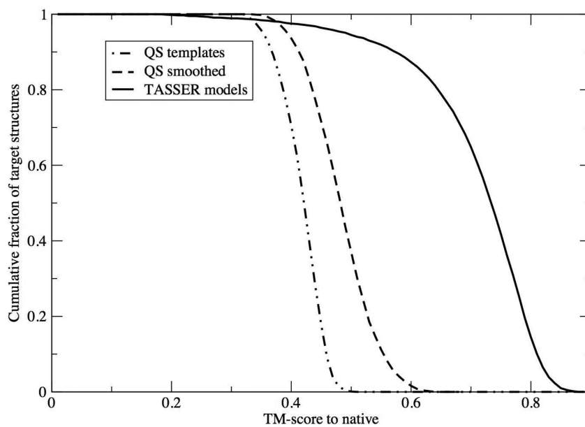
Figure 4. Cumulative fraction of target structures whose best QS template (dot-dot-dashed), smoothed (dashed) and first ranked TASSER model has a TM score value on the abscissa.
