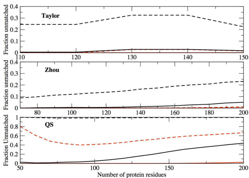
Figure 9. Fraction of unmatched targets in the Taylor, Zhou and QS sets to the PDB library as a function of the number of target protein residues. Red (black) indicates a TM-score threshold of 0.45 (0.50). Dashed (solid) lines are for the original (smoothed) structure.
