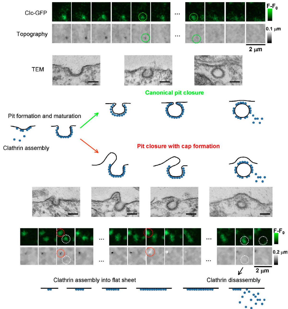
Figure 4. Proposed model of different CCP closure types. Clathrin molecules upon attachment to the membrane either start nucleating into a CCP or form a flat sheet. Once the CCP has gone through its maturation process, it can close with (red circles) or without (green circles) a cap. In some cases, Clc-EGFP fluorescence spots can be seen without associated topographically detected pits (white circles) that most likely represent flat sheets of clathrin. Bars, 100 \mu\text{m} in all TEM images.
