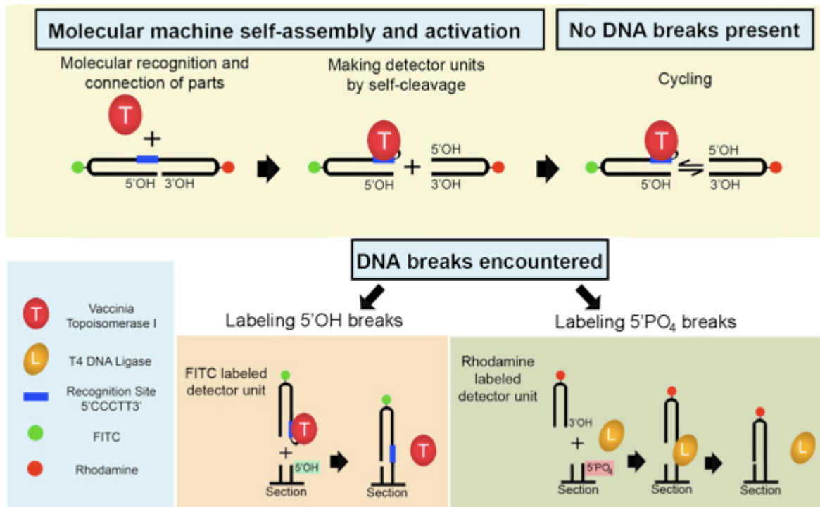
Figure 1. Semi-artificial molecular machine detects two types of DNA damage in situ . The fluorescent machine self-assembles when VACC TOPO binds to the double-hairpin 32-mer. The machine begins operation by splitting itself into two detector units via topoisomerase-made cut at the 3' end of the recognition sequence. This results in a cyclic process where the FITC-labeled unit continuously separates and religates back to the rhodamine-labeled unit. This persists until a detectable DNA break is encountered. When such an alternative acceptor (5'OH blunt end DNA break) is present in the tissue section, the FITC part will ligate to it. The remaining rhodamine part will attach to 5' PO 4 DNA blunt end breaks with the help of T4 DNA ligase. Consequently, both types of DNA breaks are simultaneously detected.
