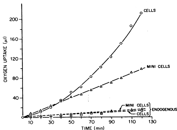
FIG. 2.—Oxygen consumption by cells and minicells of E. coli P678-54 culture: Warburg vessels contained in the main compartment 3 \times 10^8 cells (O—O) or 1 \times 10^{10} minicells (Δ—Δ) suspended in 2.6-ml minimal media and 0.2 ml of 1 N NaOH in the center well. At time 0, 0.2 ml of 20% glucose (—) or water (—) was added to the main compartment.
