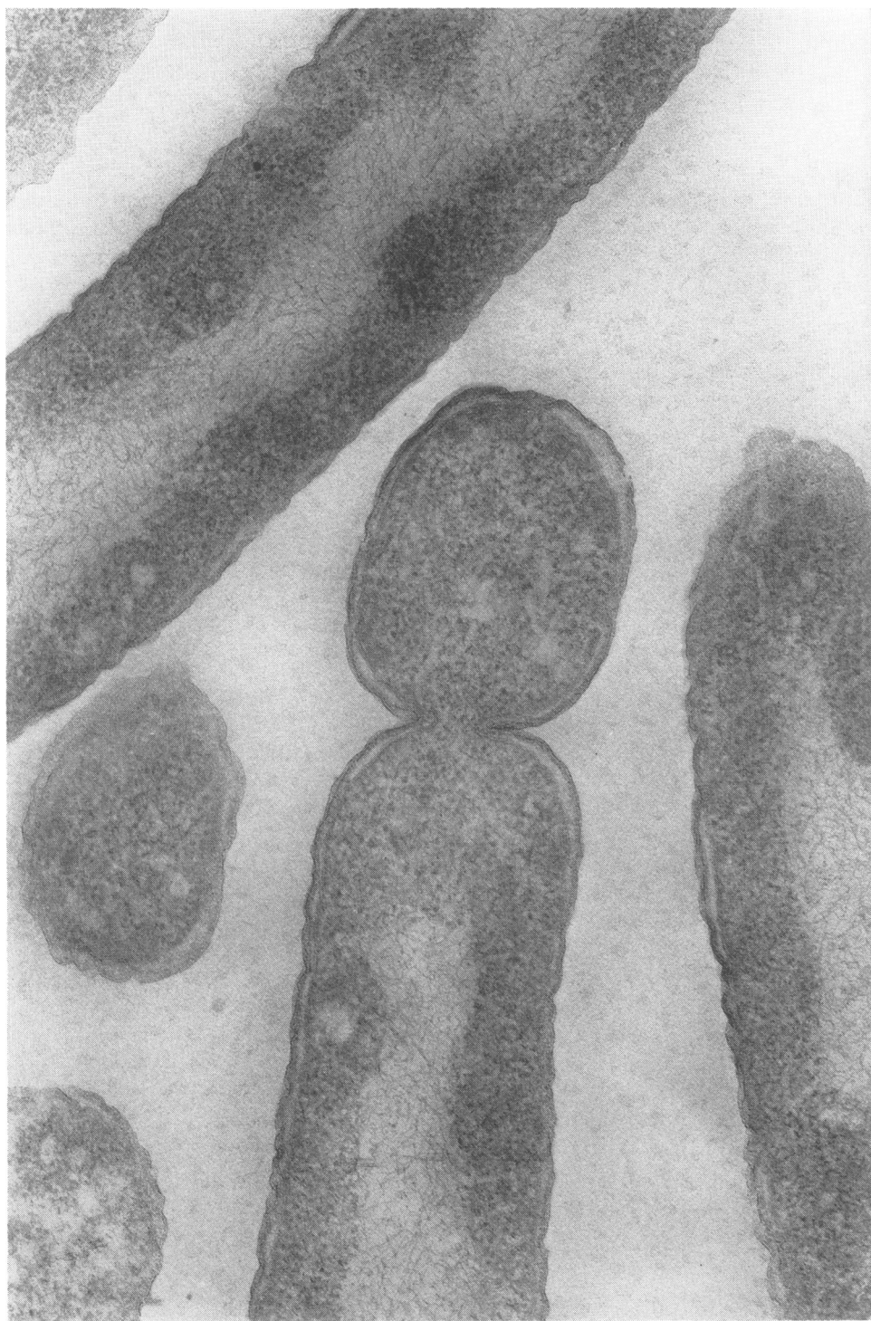
FIG. 1.—Thin-section electron micrograph showing a cell producing a minicell. \times 66,000 .
