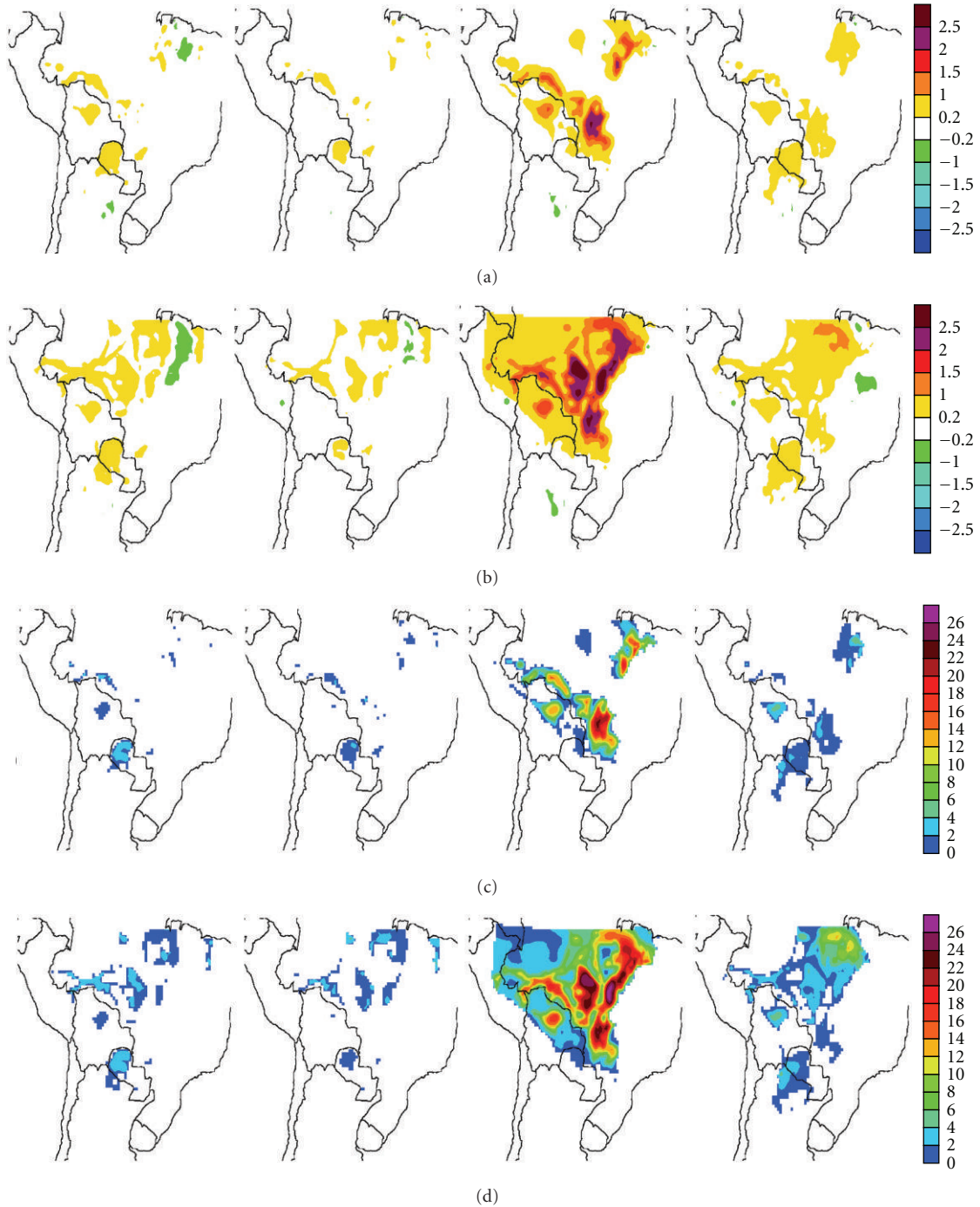
FIGURE 10: Seasonal temperature changes, in °C, resulting from the two deforestation/land-use scenarios in ECHAM-4 Baseline driven PRECIS runs, for (a) MAP1 and (c) MAP2. The corresponding significances at least at the 95% level are shown in (b) and (d), respectively. Starting from the left the columns correspond to summer (DJF), autumn (MAM), winter (JJA), and spring (SON).
