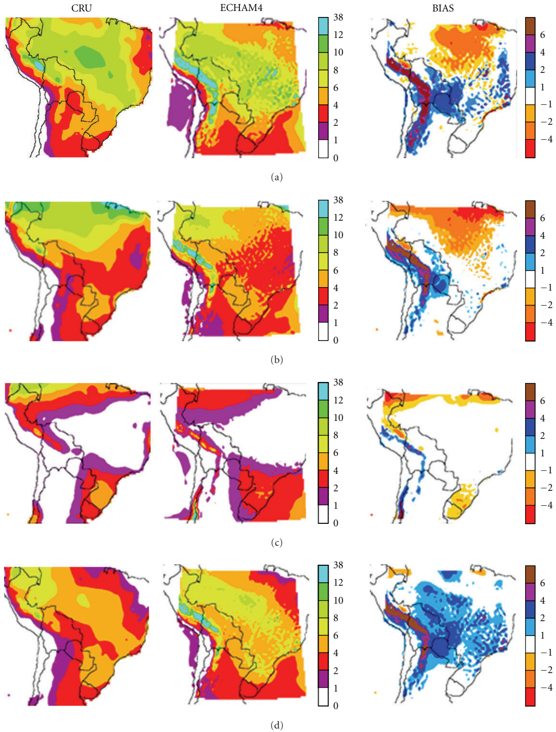
FIGURE 4: CRU fields (left column) and CONTROL-EC4 (center column) seasonal precipitation, given as precipitation rate (mm day -1 ) for (a) summer (DJF), (b) autumn (MAM), (c) winter (JJA) and (d) spring (SON). The bias, that is, CONTROL-EC4 minus CRU, is shown in the right column.
