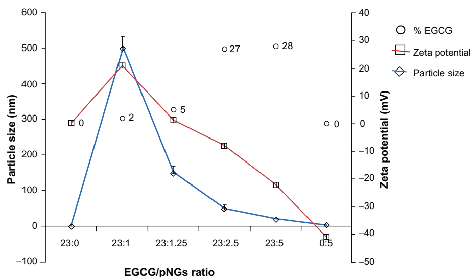
Figure 2 The characteristics of EGCG-pNG particles show the percentage of EGCG capped on pNGs (O), particle size (◇), and zeta potential (□) at different ratios of EGCG:pNG (23:0, 23:1, 23:1.25, 23:2.5, 23:5, and 0:5).
